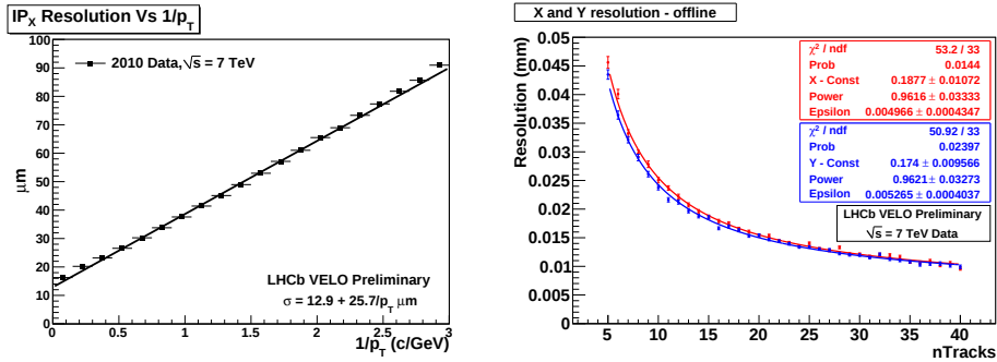
Fig. 4. The left-hand histogram shows the \text{IP}_X resolution as a function of 1/p_T . The right-hand histogram shows the \text{PV}_X (red) and \text{PV}_Y (blue) resolutions as a function of the track multiplicity.
