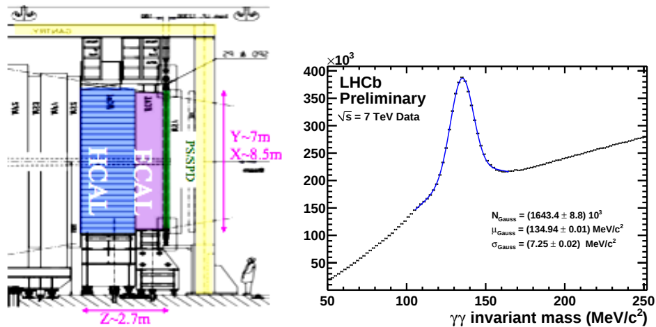
Fig. 8. The left-hand picture shows a sketch of the LHCb calorimeter system. The right-hand histogram shows the invariant mass of two \gamma s reconstructed in the electromagnetic calorimeter.
