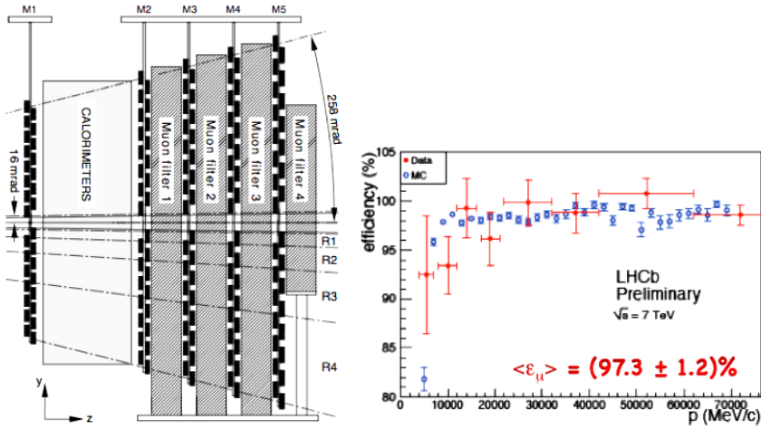
Fig. 10. The left-hand picture shows a sketch of the LHCb muon system. The right-hand histogram shows the muon identification efficiency as a function of the muon momentum.
