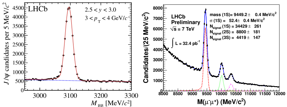
Fig. 11. The left-hand histogram shows the J/\psi invariant mass from the \mu^+\mu^- decay channel [5]. The right-hand histogram shows the invariant masses of the \Upsilon resonances, \Upsilon(1S) , \Upsilon(2S) and \Upsilon(3S) from left to right. The superimposed curves on the signal and the yields are the result of a fit described in [6].
