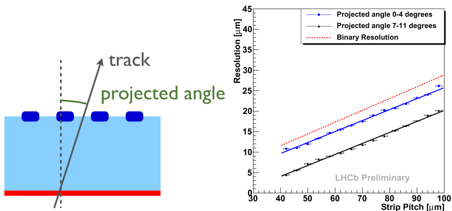
Fig. 3. The left picture shows a sketch of the projected angle. The right-hand histogram shows the VELO hit resolution versus the strip pitch in two projected angle regions.
