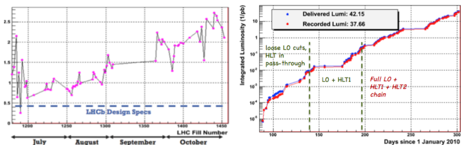
Fig. 2. The left-hand histogram shows the behavior of \mu from July 2010 to the end of the data taking period compared to the design value. The right-hand histogram shows the integrated luminosity delivered (blue) and collected (red) during the 2010.
