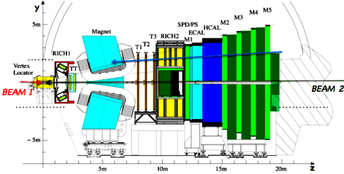
Fig. 1. Schematic view of the LHCb detector.
