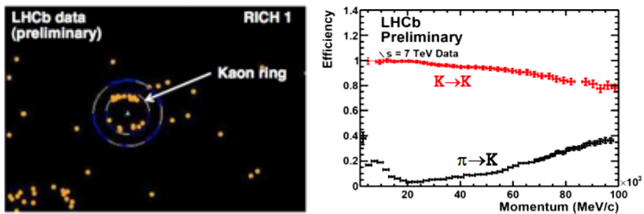
Fig. 7. The left-hand picture shows the Cherenkov light: the (orange) points. The right-hand histogram shows the RICH K/\pi separation performance as a function of the momentum.
