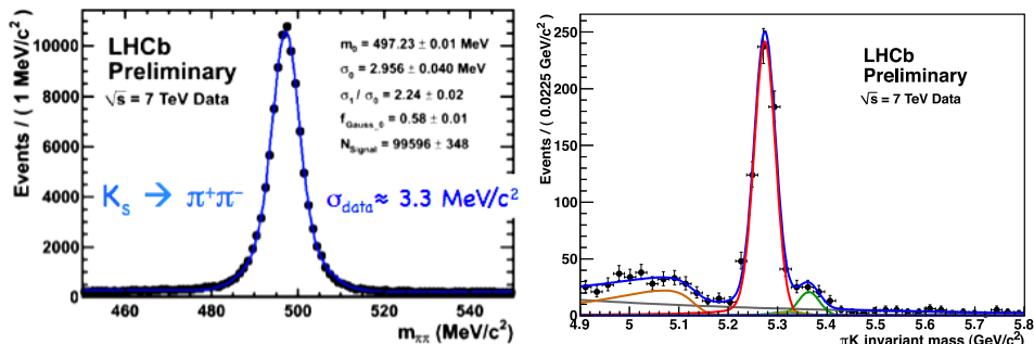
Fig. 5. The left-hand histogram shows the mass invariant for K_S \rightarrow \pi\pi , while the right-hand histogram shows the mass invariant for B \rightarrow K\pi ( \sigma \simeq 25 \text{ MeV}/c^2 ).
