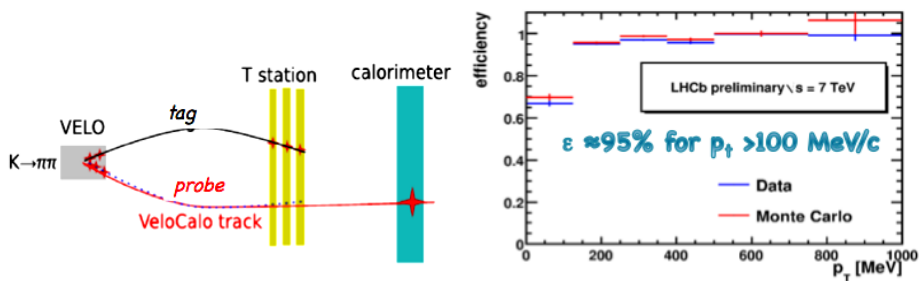
Fig. 6. The left-hand picture is a sketch to describe the tag and probe method with K_S \rightarrow \pi\pi decays. The right-hand histogram shows the tracking efficiency as a function of p_T for data (blue) and Monte Carlo (red).
