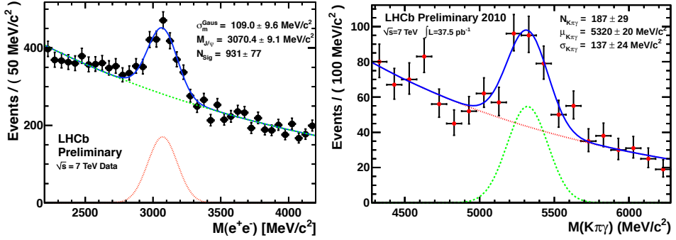
Fig. 9. The left-hand histogram shows the J/\psi invariant mass from the e^+e^- decay channel. The right-hand histogram shows the invariant mass of the B meson from the radiative decay to \gamma K^* .
