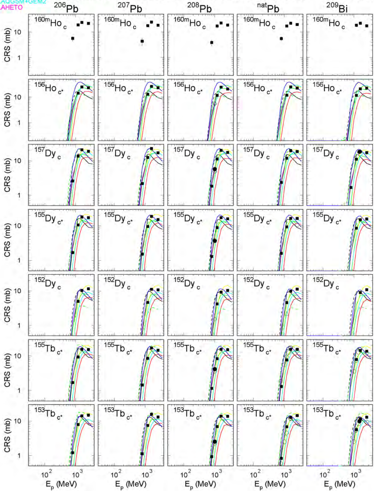
Fig. 68: The simulated and experimental cross sections of the measured reactions (Continuation of Fig. 53).
