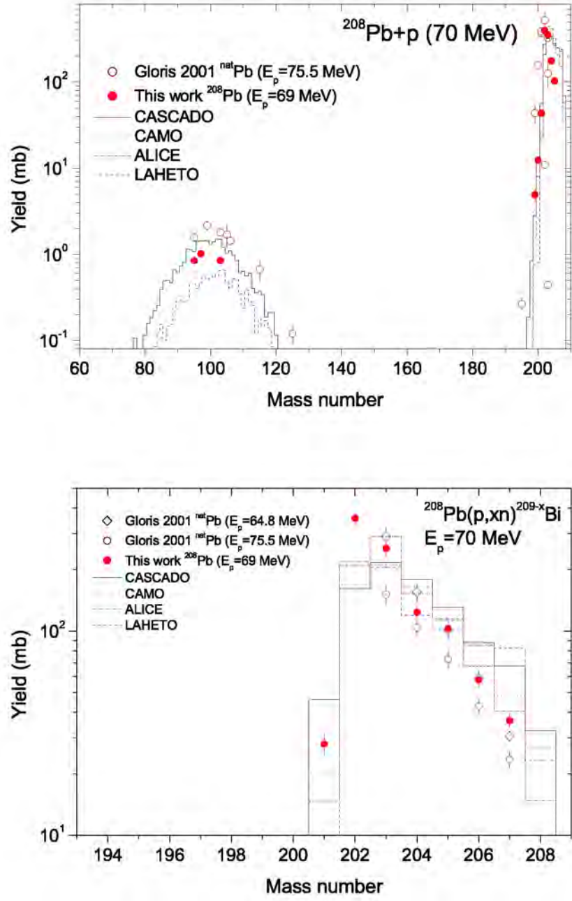
Fig. 50: Experimental data on cumulative yields of spallation and fission products and on the bismuth isotopic yields for ^{208}\text{Pb} target irradiated by 70 MeV protons compared with cascade-model calculations.
