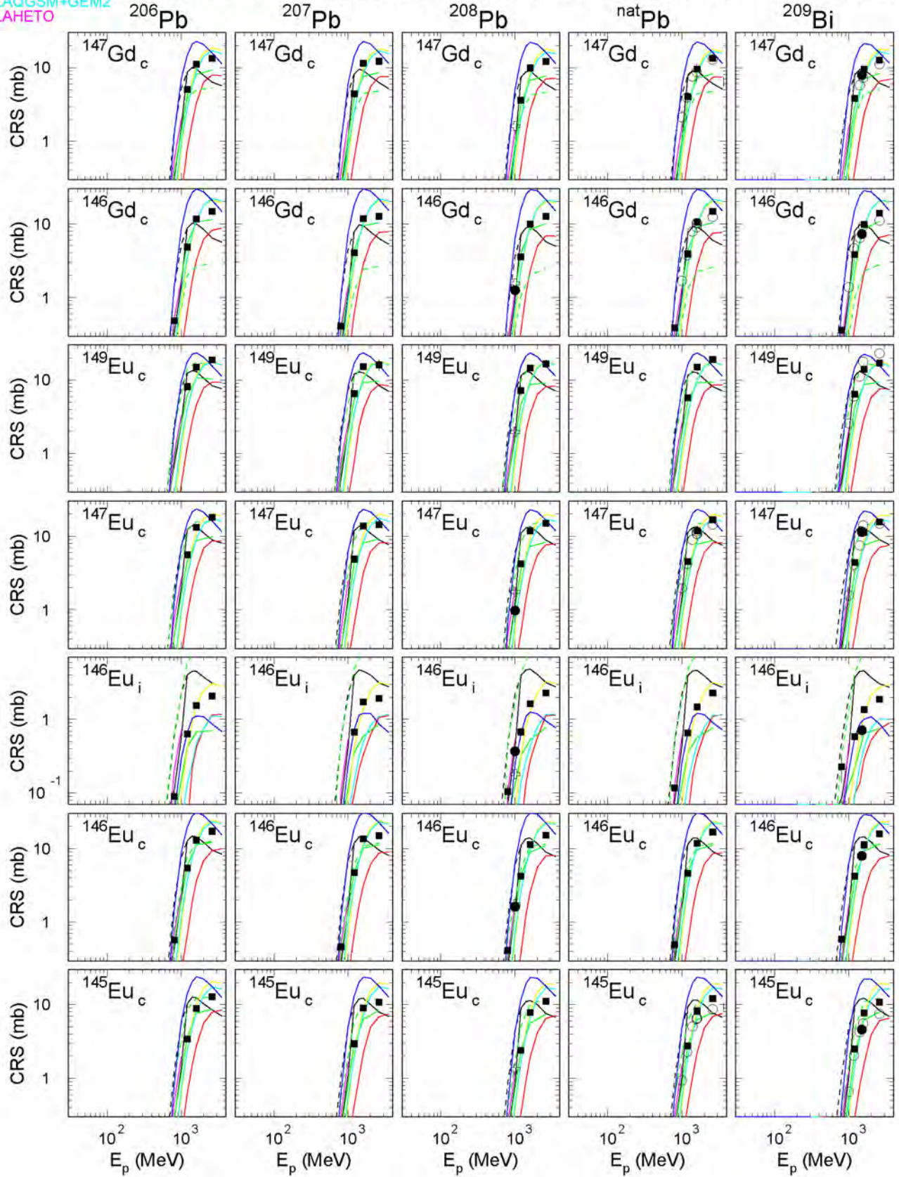
Fig. 70: The simulated and experimental cross sections of the measured reactions (Continuation of Fig. 53).
