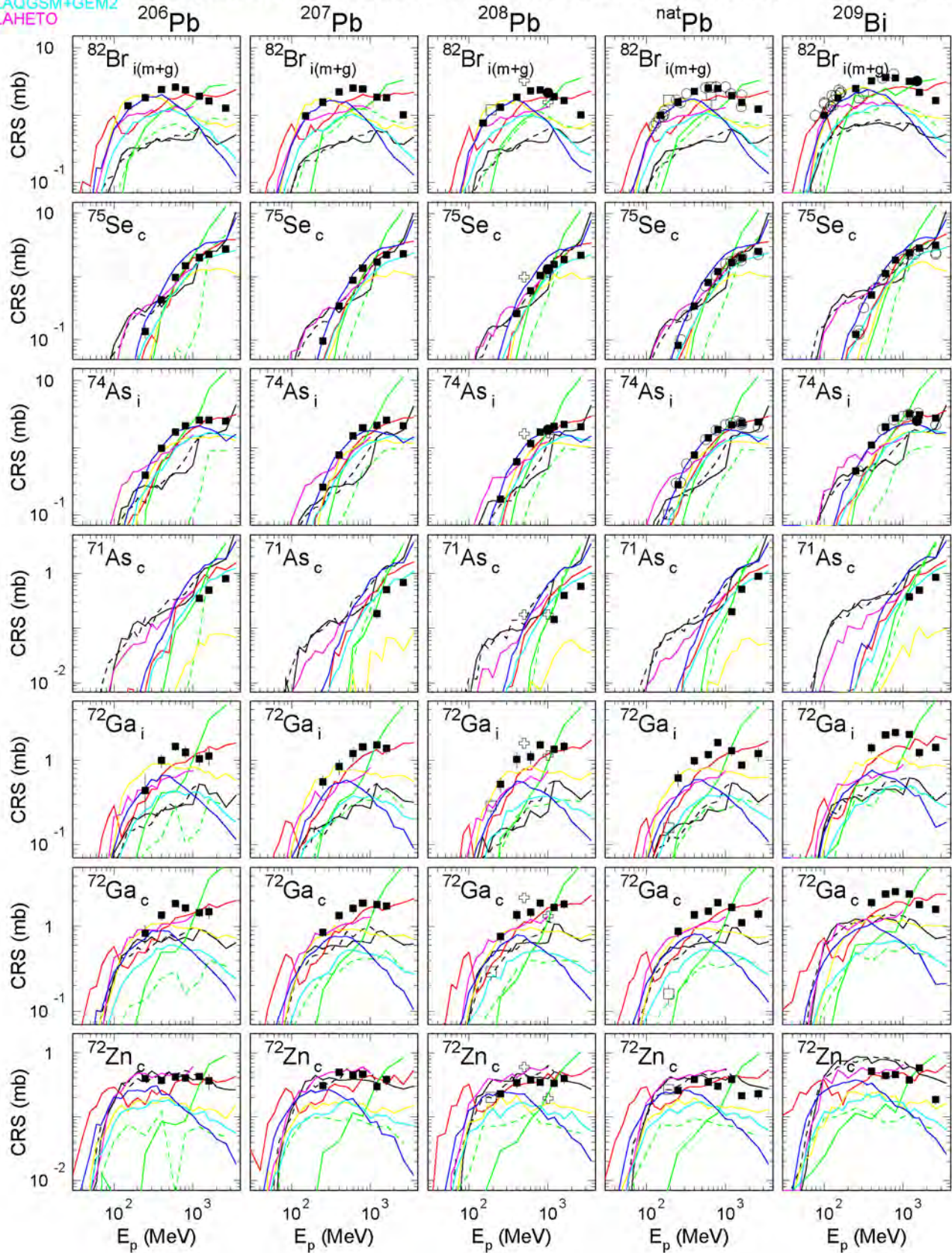
Fig. 79: The simulated and experimental cross sections of the measured reactions (Continuation of Fig. 53).
