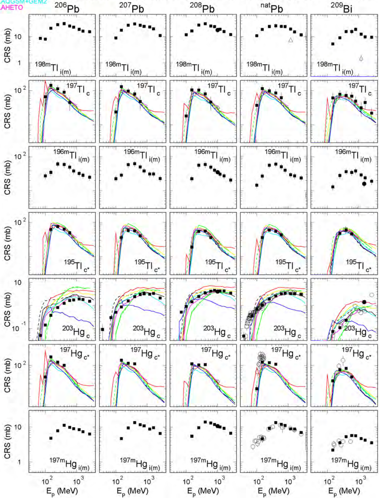
Fig. 57: The simulated and experimental cross sections of the measured reactions (Continuation of Fig. 53).
