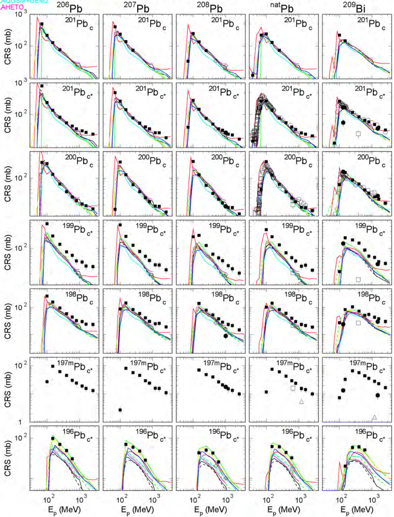
Fig. 55: The simulated and experimental cross sections of the measured reactions (Continuation of Fig. 53).
