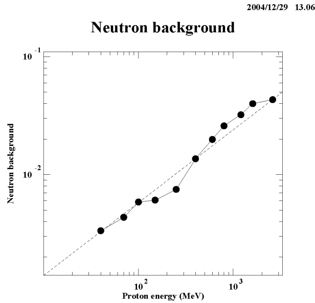
Fig. 13: The mean neutron flux-to-mean proton flux density ratio in the proton flux versus proton beam energy.
