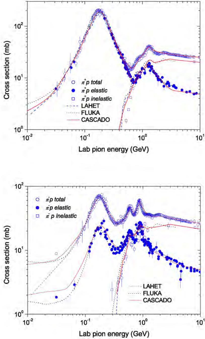
Fig. 32: Total, elastic, and inelastic cross sections for \pi^+ - p and \pi^- - p collisions used by various INCM codes in comparison with experimental data .
