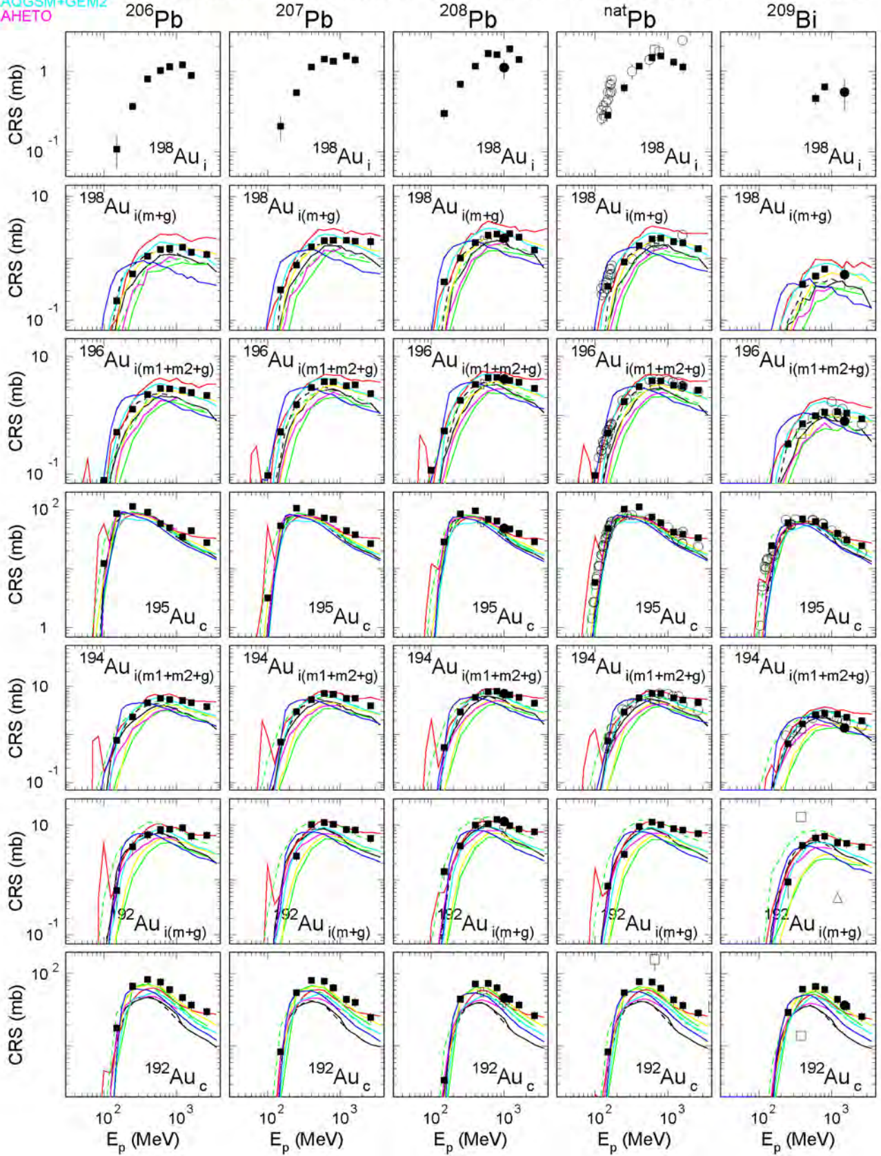
Fig. 59: The simulated and experimental cross sections of the measured reactions (Continuation of Fig. 53).
