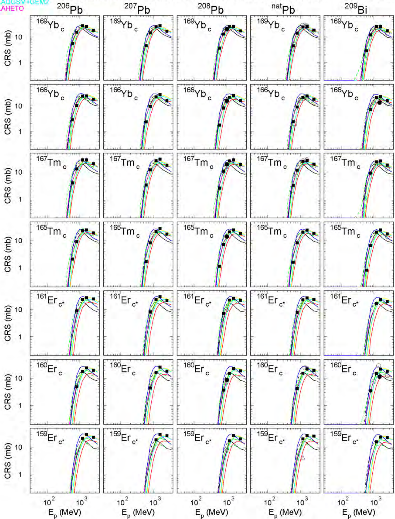
Fig. 67: The simulated and experimental cross sections of the measured reactions (Continuation of Fig. 53).
