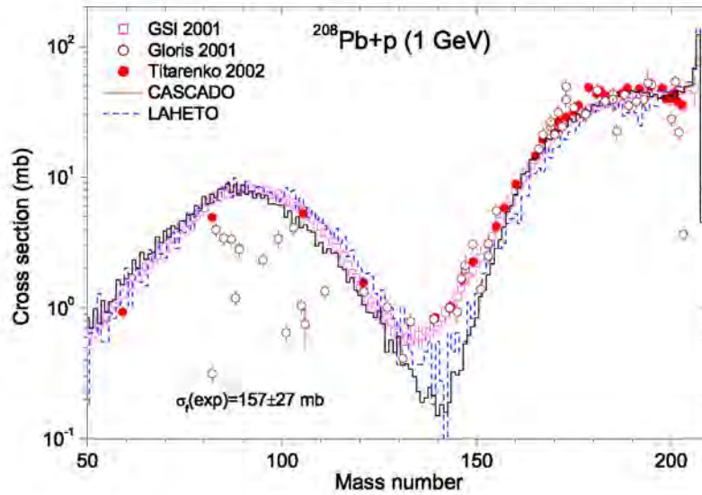
Fig. 38: Experimental data on the residual-mass distribution (open squares) and residual cumulative yields (solid circles) for the ^{208}\text{Pb}+p(1 \text{ GeV}) reaction in comparison with cascade-model calculations.
