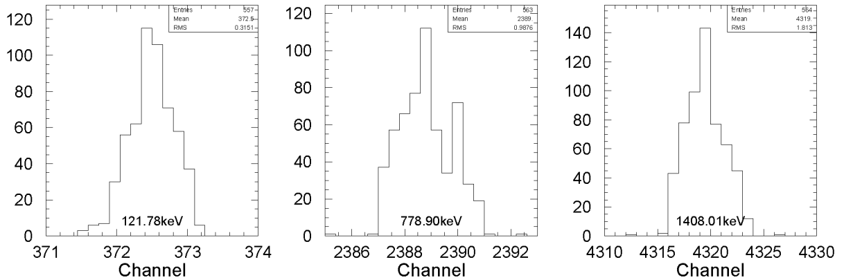
Fig. 15: General statistics of the spectrometer time stability.
