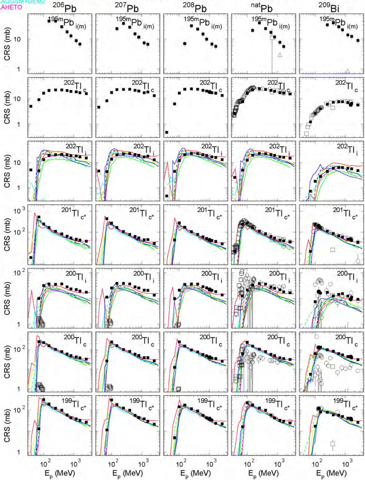
Fig. 56: The simulated and experimental cross sections of the measured reactions (Continuation of Fig. 53).
