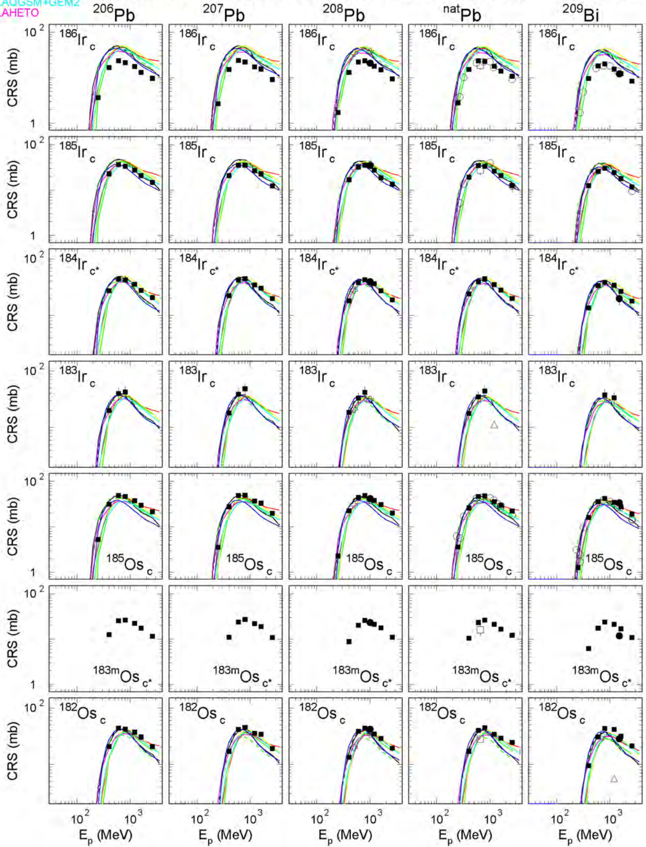
Fig. 62: The simulated and experimental cross sections of the measured reactions (Continuation of Fig. 53).
