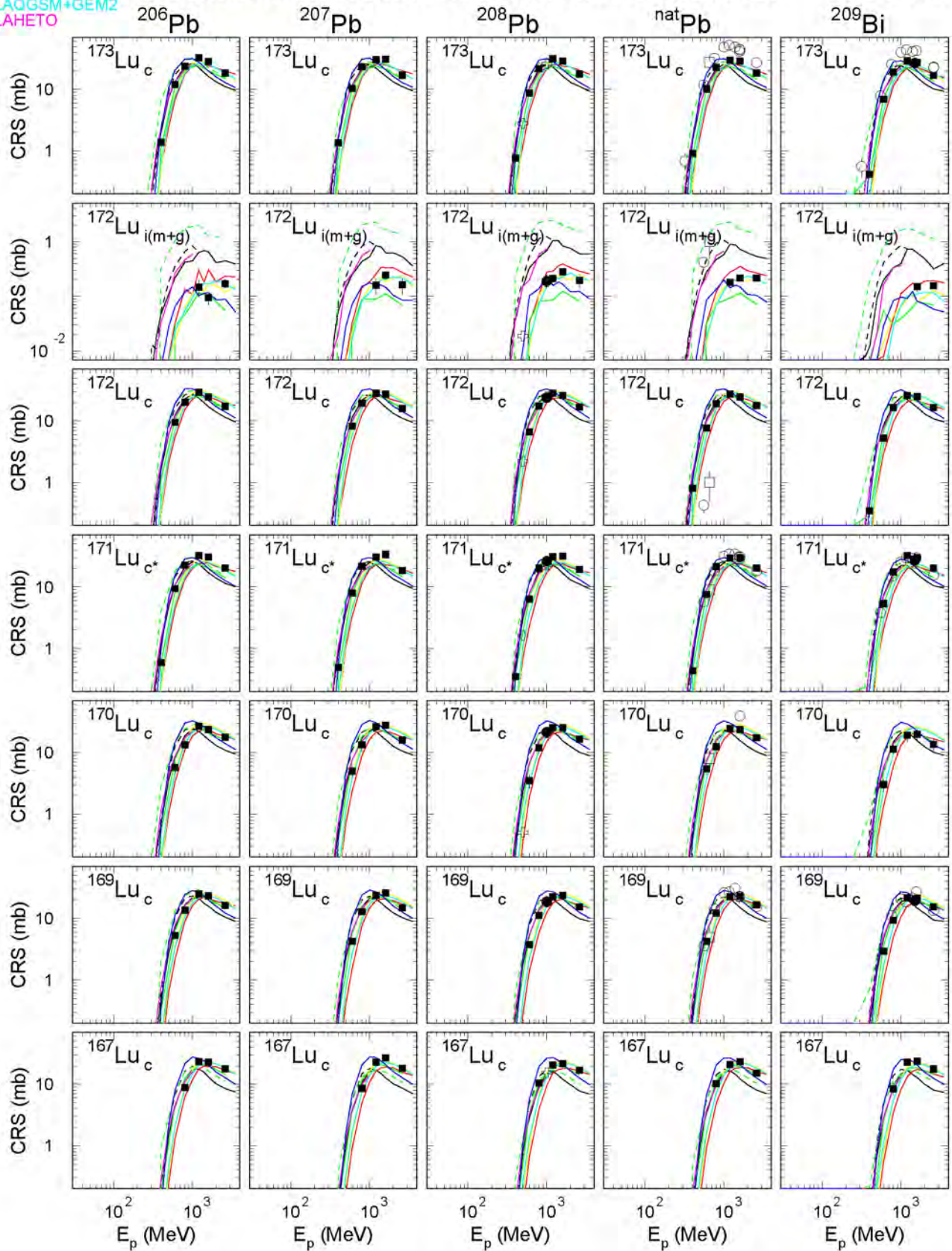
Fig. 66: The simulated and experimental cross sections of the measured reactions (Continuation of Fig. 53).
