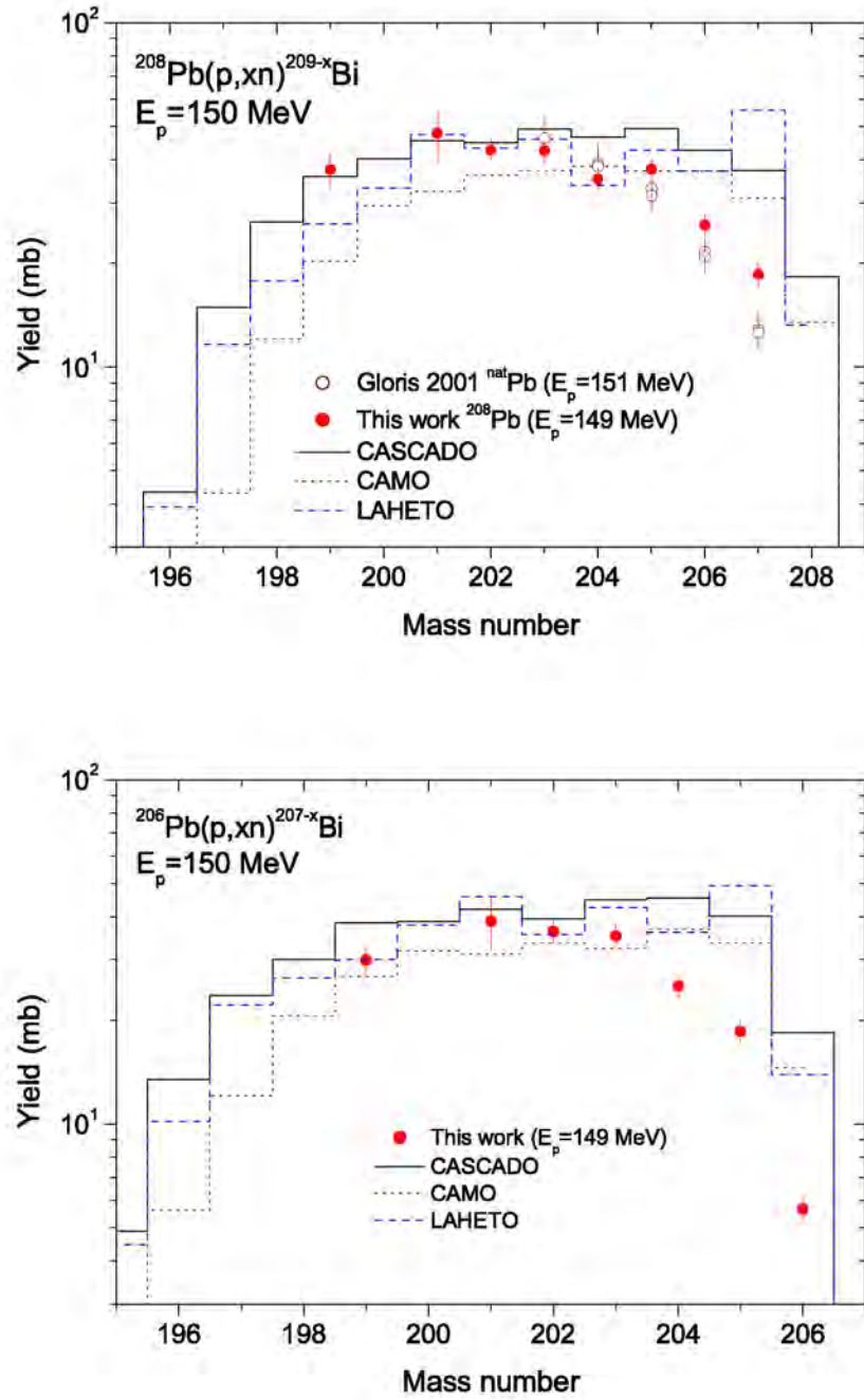
Fig. 48: Experimental data on the bismuth isotopic yields for ^{208}\text{Pb} and ^{206}\text{Pb} targets irradiated by 150 MeV protons compared with cascade-model calculations.
