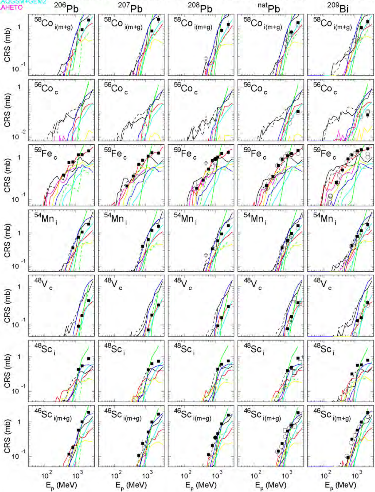
Fig. 80: The simulated and experimental cross sections of the measured reactions (Continuation of Fig. 53).
