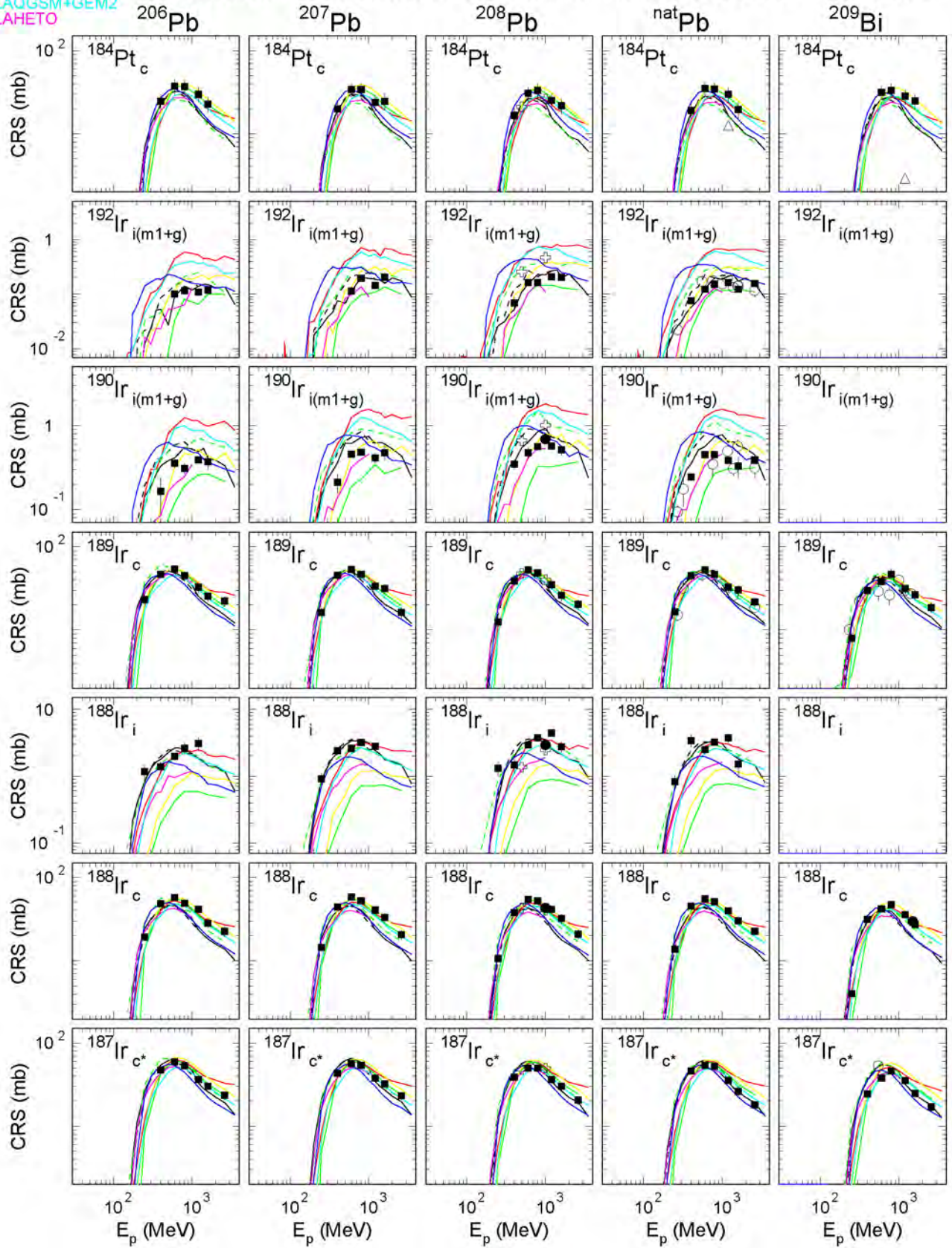
Fig. 61: The simulated and experimental cross sections of the measured reactions (Continuation of Fig. 53).
