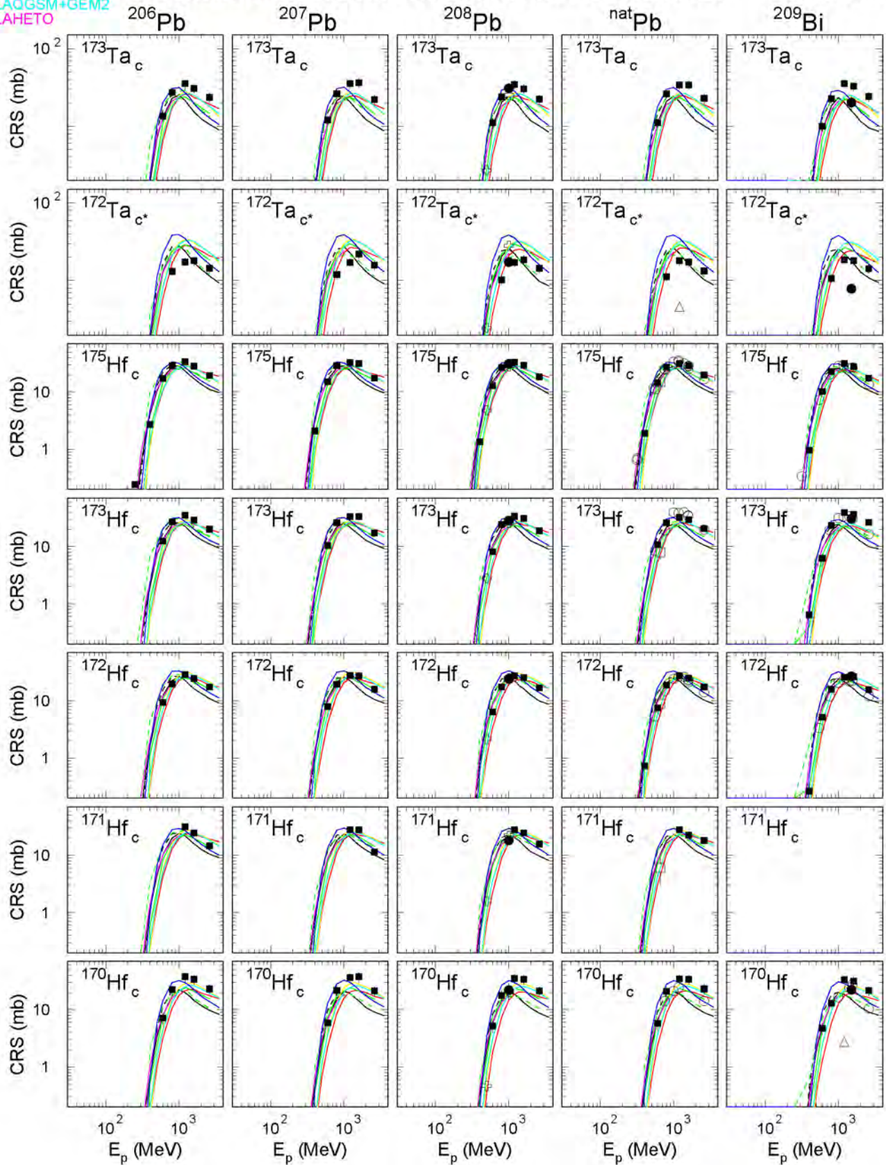
Fig. 65: The simulated and experimental cross sections of the measured reactions (Continuation of Fig. 53).
