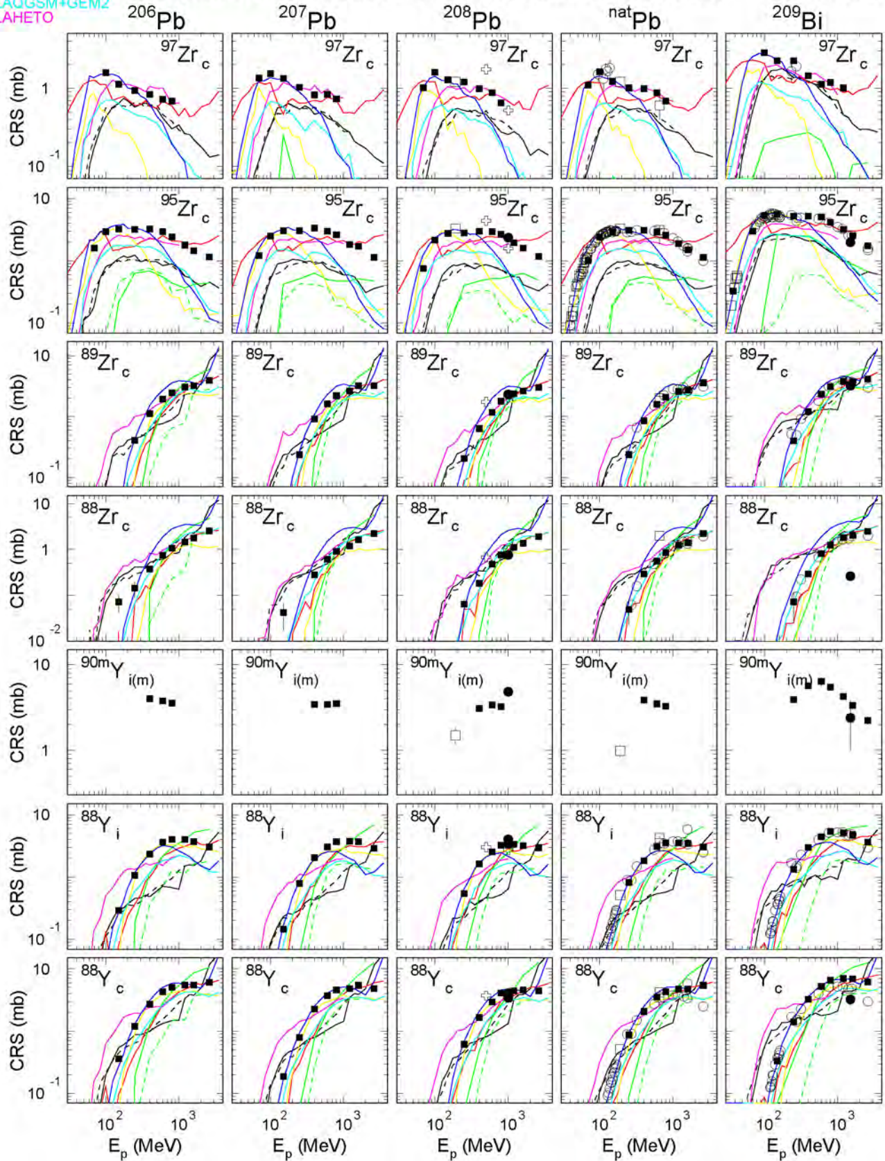
Fig. 77: The simulated and experimental cross sections of the measured reactions (Continuation of Fig. 53).
