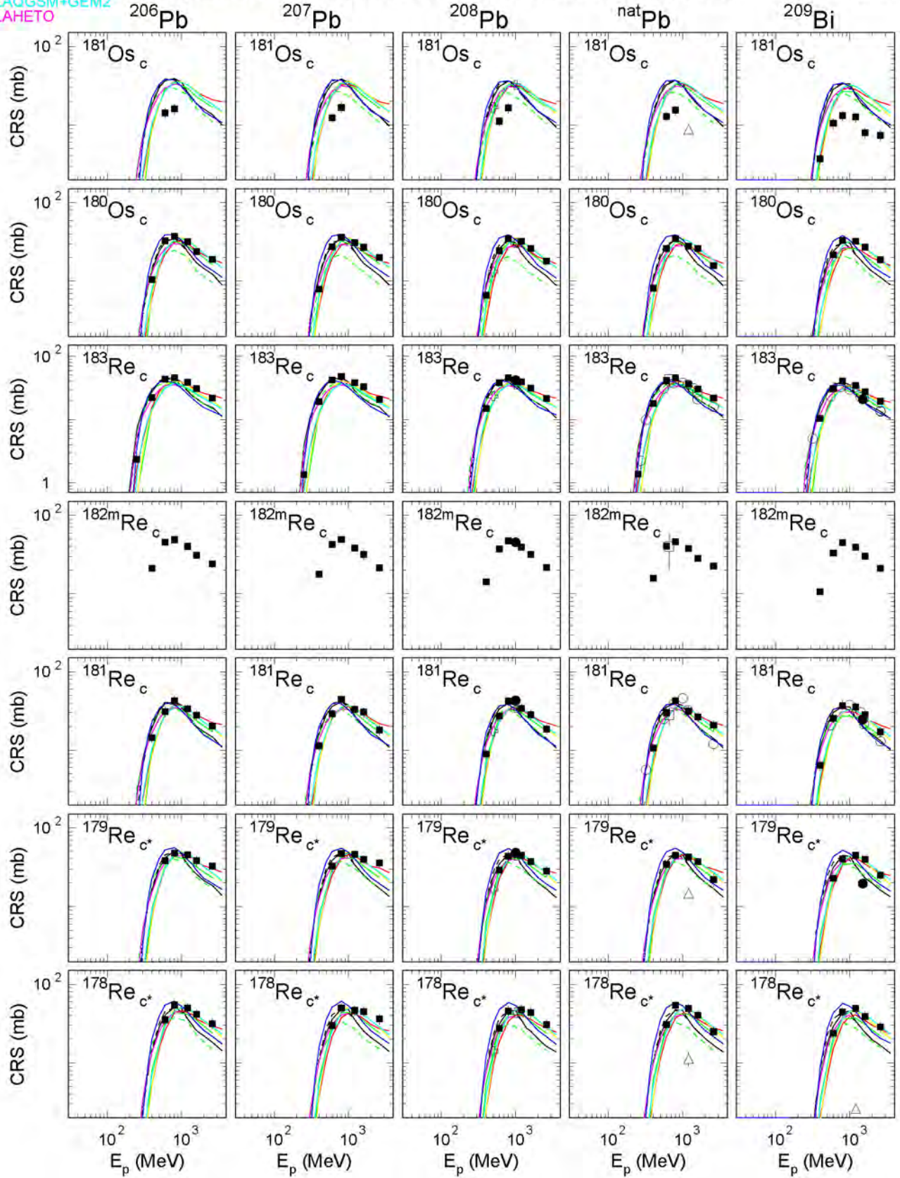
Fig. 63: The simulated and experimental cross sections of the measured reactions (Continuation of Fig. 53).
