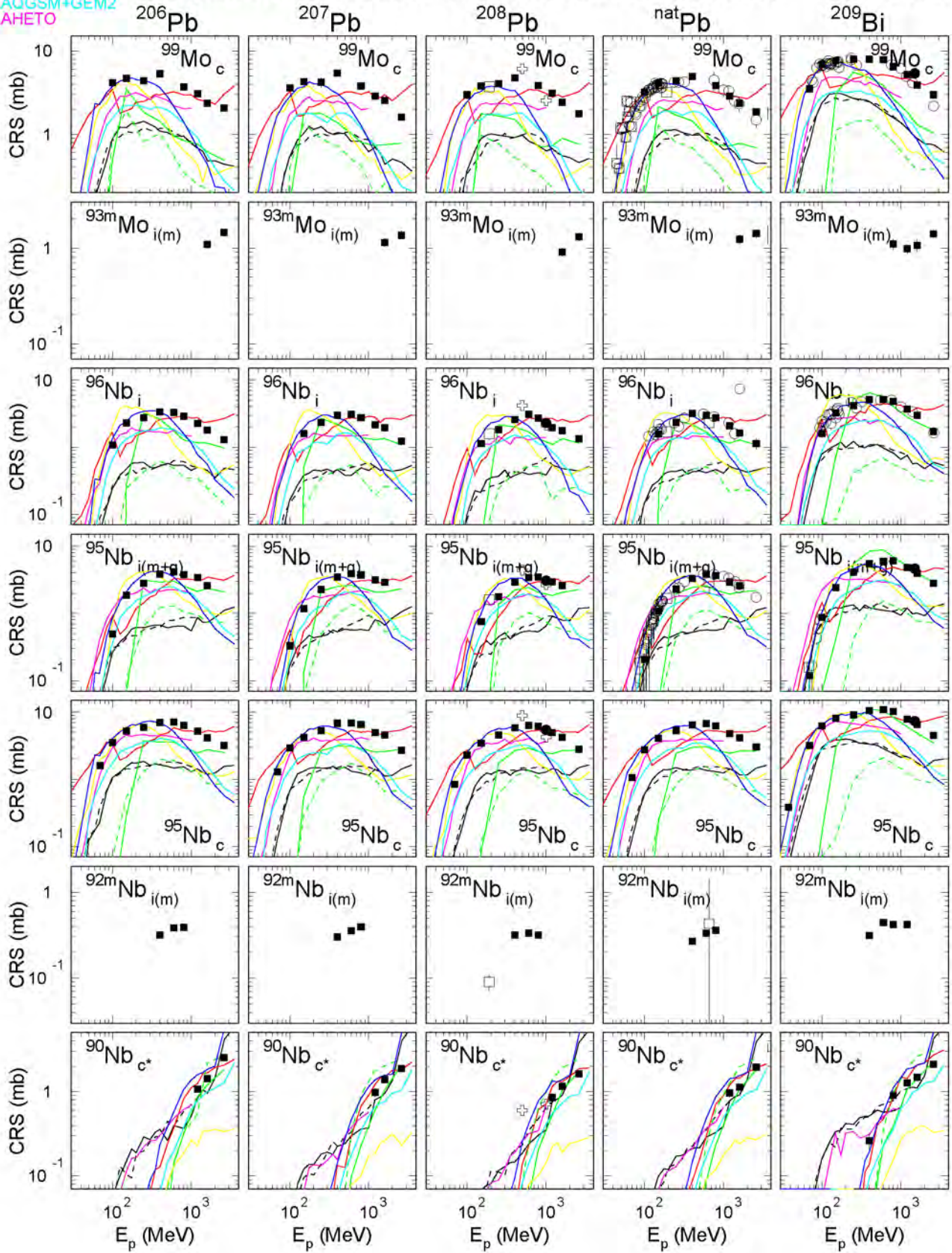
Fig. 76: The simulated and experimental cross sections of the measured reactions (Continuation of Fig. 53).
