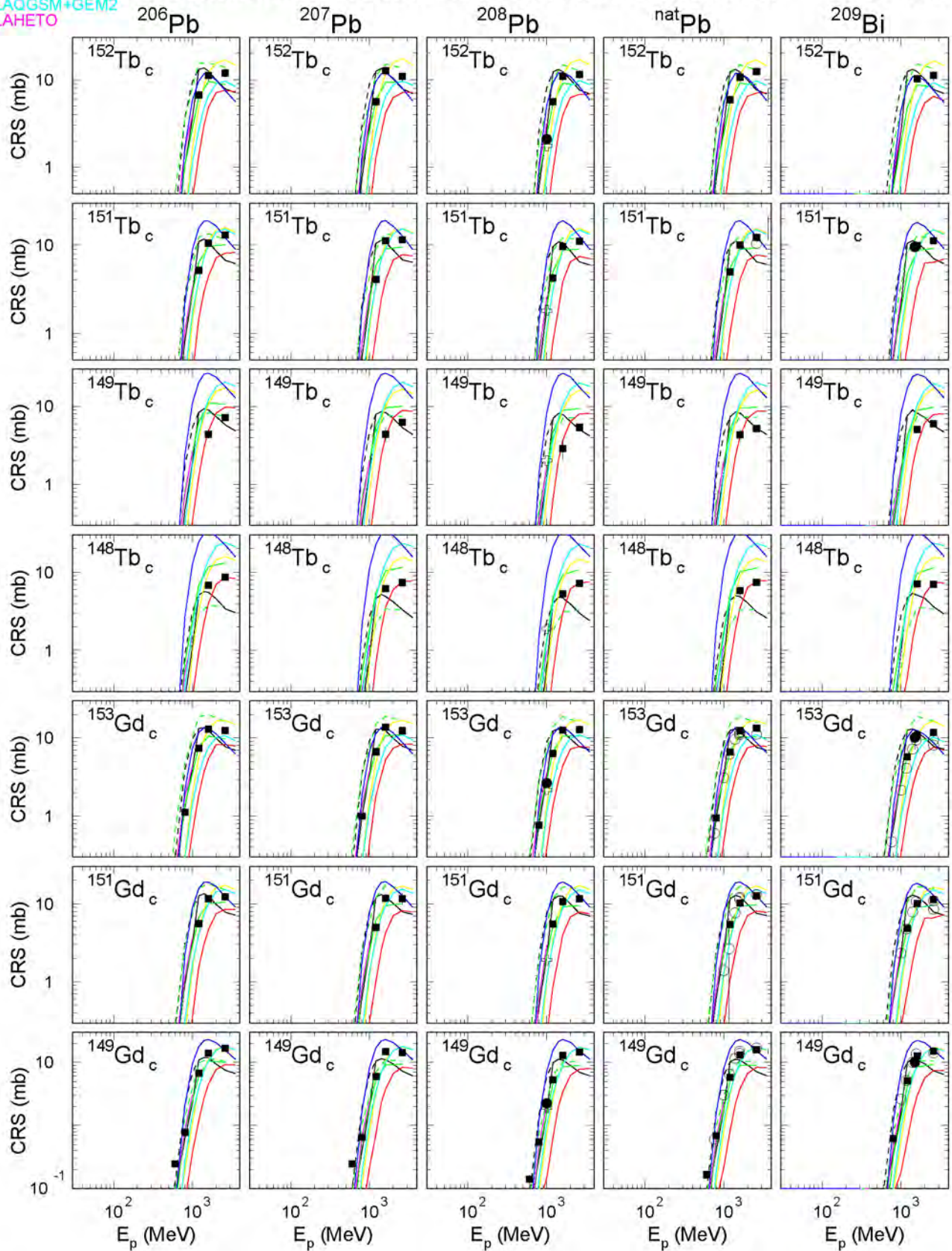
Fig. 69: The simulated and experimental cross sections of the measured reactions (Continuation of Fig. 53).
