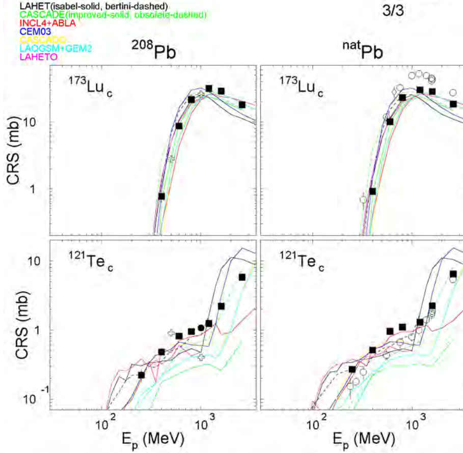
Fig. 28: Comparison with the results obtained elsewhere: ^{173}\text{Lu} and ^{121}\text{Te} . ■ - This Report, ○ - [117, 105, 82, 108], ◇ - [83, 93], open star - [56, 90], + - [123, 102], star - [106], • - [6], □ - [94]
