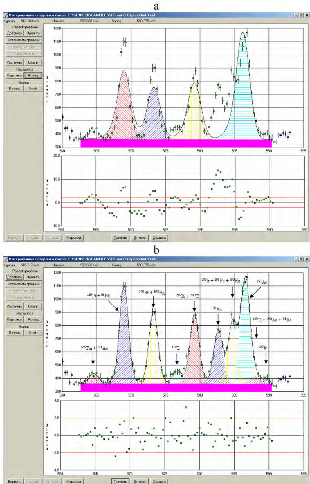
Fig. 20: The results of primary processing a \gamma -spectrum by the automatic (a) and manual interactive fitting(b) modes of the GENIE-2000 code.
