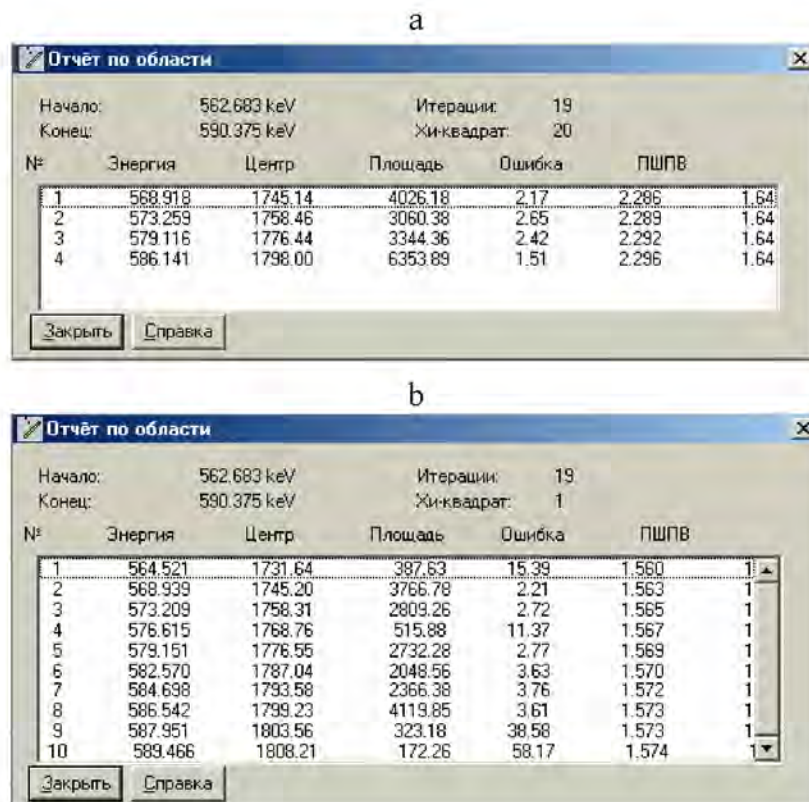
Fig. 21: The GENIE-2000 report on the parameters of the found peaks. The legend (a) and (b) is the same as in Fig. 20.
