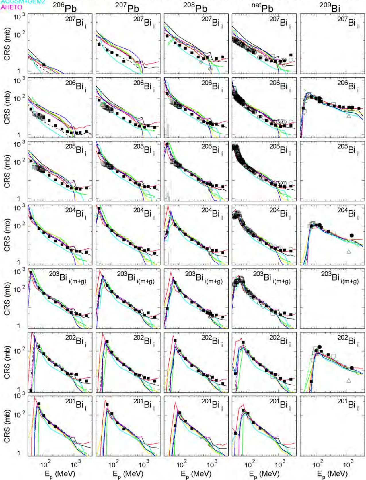
Fig. 53: The simulated and experimental cross sections of the measured reactions (■ - this work, + - [123], ○ - [117], ● - [6, 4], △ - [101], ▮ - other works; LAHET - black (ISABEL - solid, BERTINI - dashed), CEM03 - blue, INCL4+ABLA - red, CASCADE - green, LAQGSM03 - cyan, LEHETO - magenta, CASCADO - yellow.
