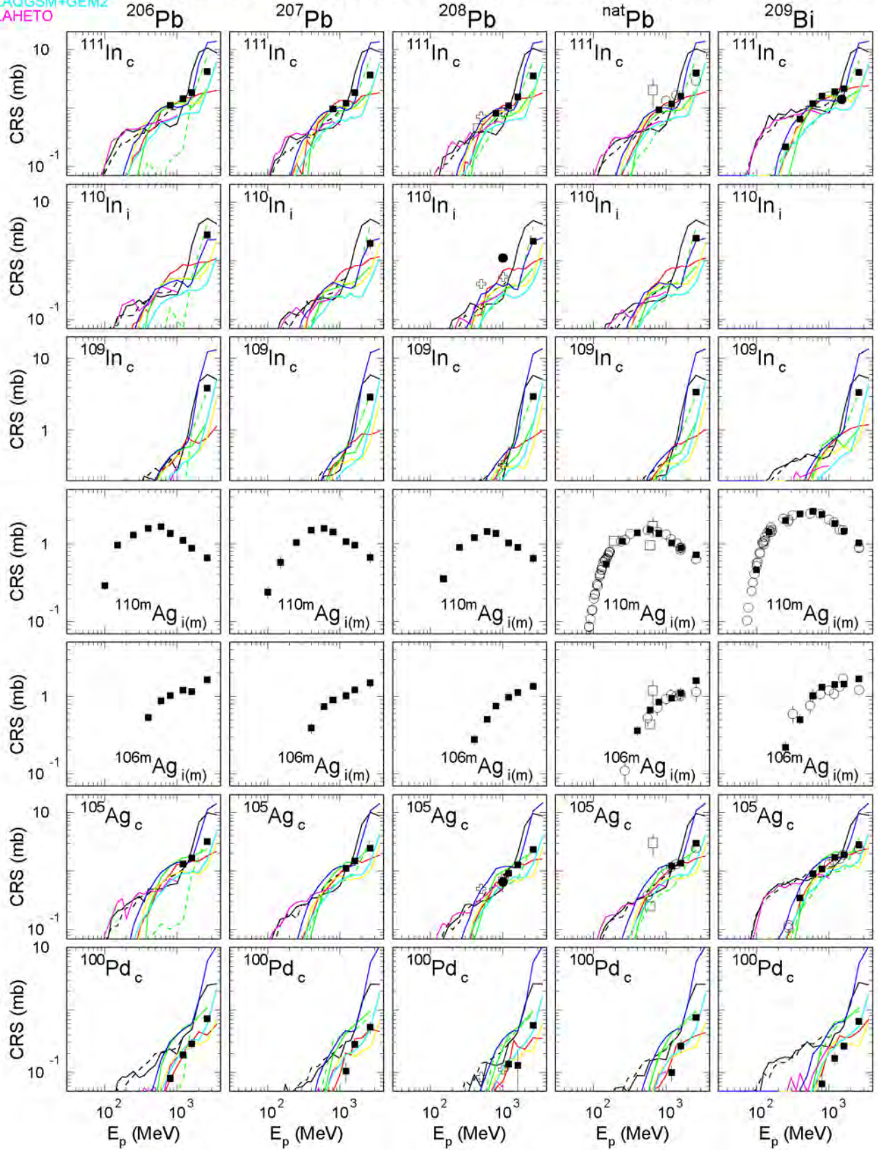
Fig. 74: The simulated and experimental cross sections of the measured reactions (Continuation of Fig. 53).
