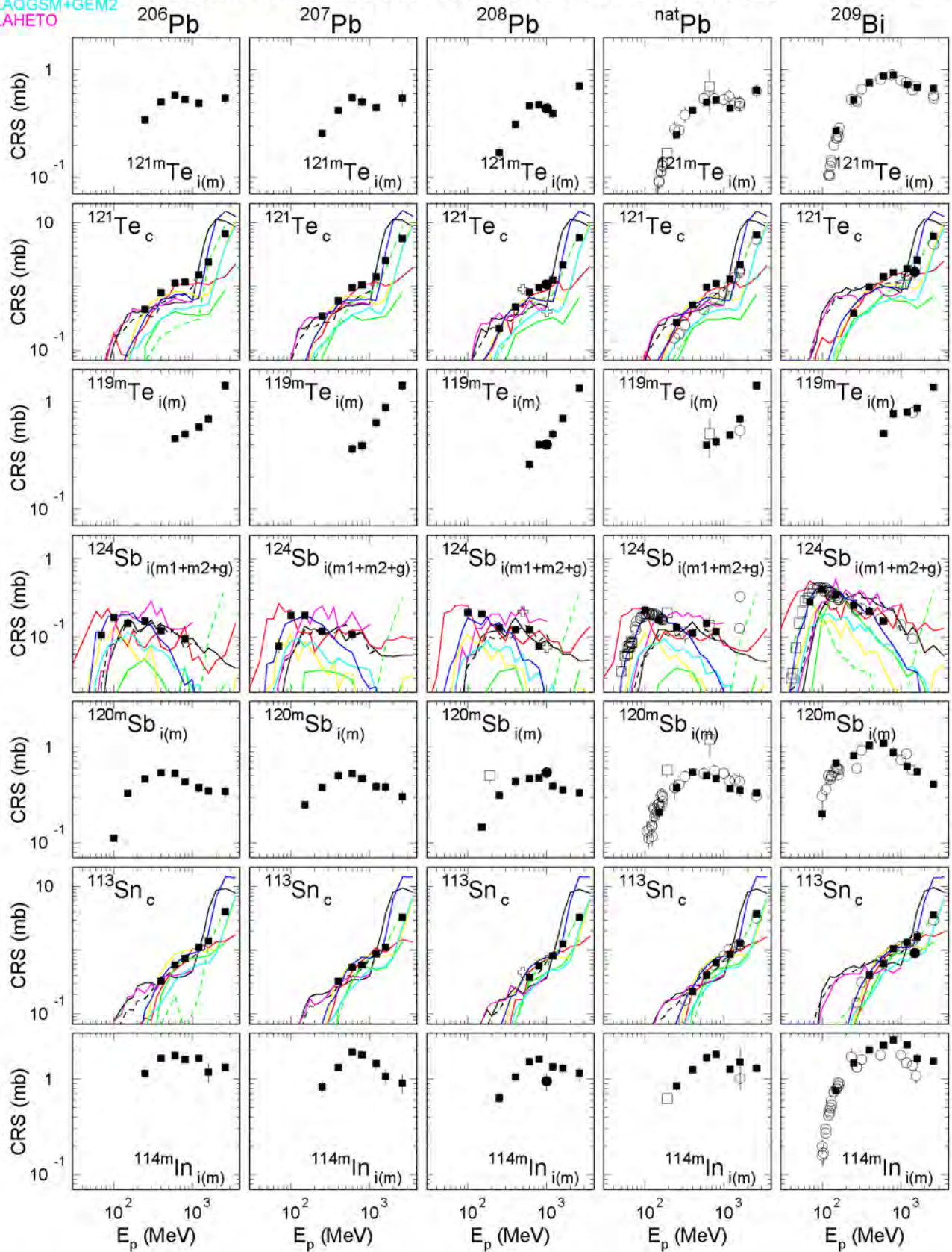
Fig. 73: The simulated and experimental cross sections of the measured reactions (Continuation of Fig. 53).
