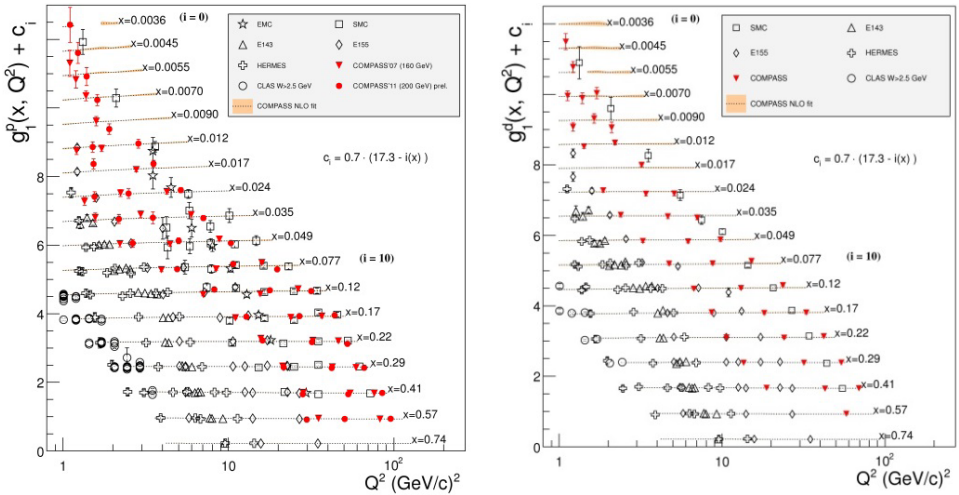
Fig. 3. World data on g_1 proton (left) and deuteron (right) vs Q^2 , for various x . COMPASS data are in red. The dotted lines represent the solutions of a COMPASS global NLO QCD fit (see text).
