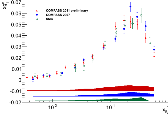
Fig. 1. Proton longitudinal spin structure function: COMPASS 200 GeV (red), 160 GeV (blue) and SMC data.
