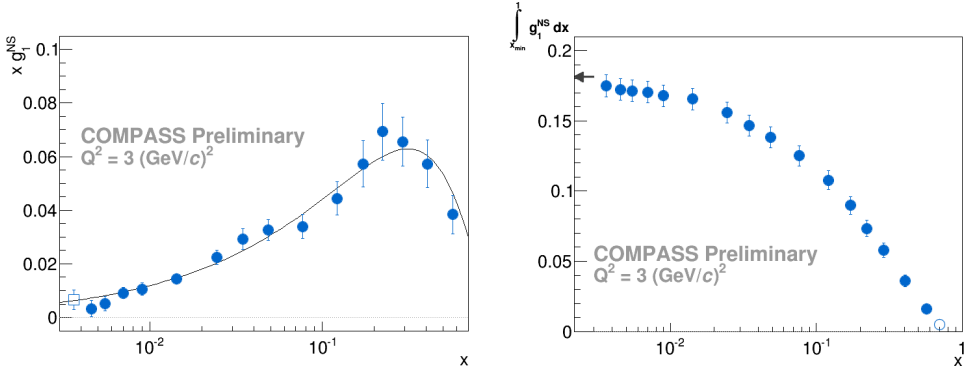
Fig. 2. Left: The nucleon non-singlet spin structure function g_1^{NS} vs x , measured from COMPASS p and d data. Right: truncated integral of g_1^{NS} from x_{\min} to 1, vs x_{\min} . The arrow shows the value extrapolated to x_{\min} = 0 .
