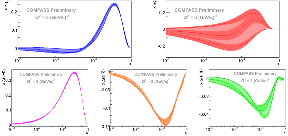
Fig. 4. Top: Helicity distributions of the quarks (left) and the gluons (right) at 3 \text{ (GeV/c)}^2 in MS scheme. Bottom: Helicity distributions per flavour. Dashed, solid and dotted lines correspond to the three solutions with positive, compatible with zero and negative DG. Dark bands correspond to propagation of statistical errors, and the light bands to the combined statistical and systematic uncertainties (dominating and mainly attributed to choice of functional forms).
