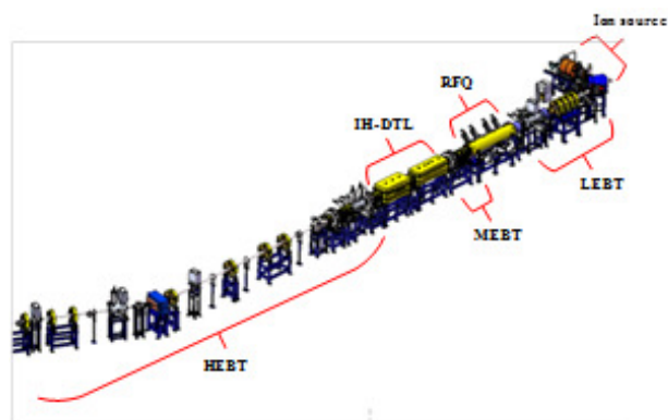
Figure 2: Layout of Linac injector.
