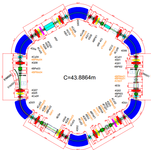
Figure 4: Layout of main ring elements.
