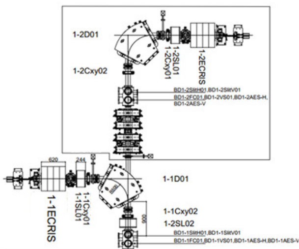
Figure 3: Layout of ion source.
