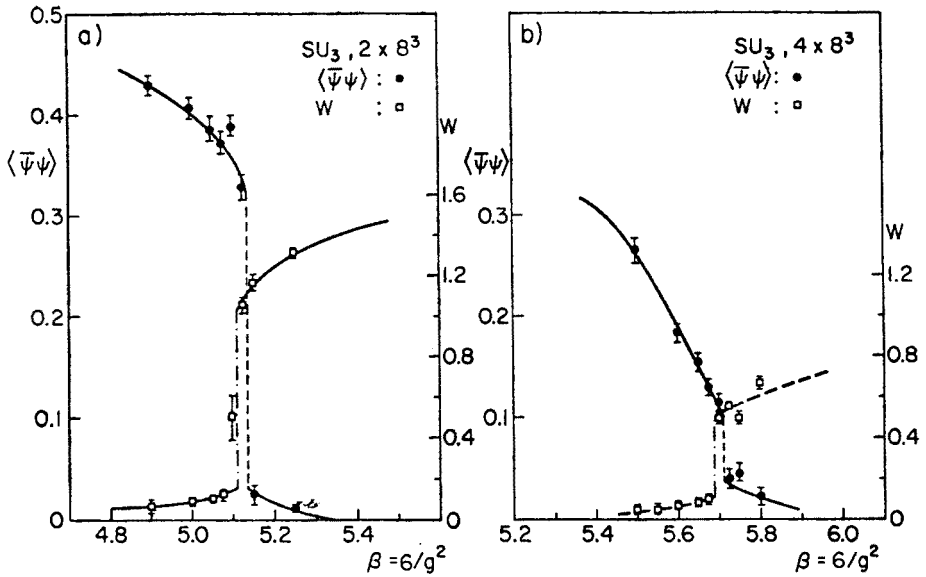
Fig. 6. The order parameters \langle \bar{\psi}\psi \rangle and \langle W \rangle in SU(3) lattice gauge theory with fundamental quarks
