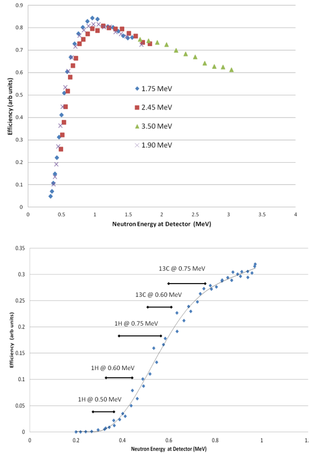
Figure 2. Neutron detector efficiency. (top) Detector efficiency determination from 3 H(p,n) measurements at four proton energies. (bottom) Detector efficiency measurements emphasizing the <1 MeV region. The kinetic ranges of several measurements spanning 30° to 150° are indicated with bars. In the case of 0.5 MeV neutrons, the energy range is too low to trust the results from a H(n,n) cross-section normalization, hence the need to use a natural carbon sample.
