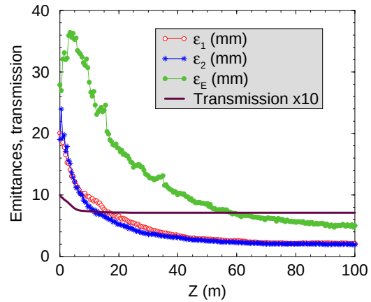
Figure 1: Normalized rms emittances and transmission vs longitudinal coordinate. 1-2 are transverse eigenmodes.
