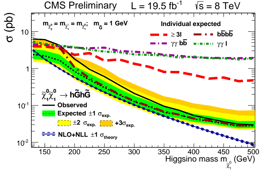
FIGURE 4. The expected and observed upper limits on the cross section of the \tilde{\chi}^0_1 \tilde{\chi}^0_1 production for HH + \vec{E}_T^{\text{miss}} studies [10].
