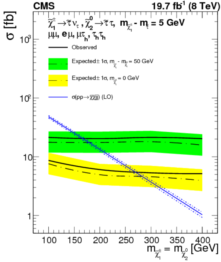
FIGURE 6. The exclusion limit on the cross section of this process vs. the \chi^{pm} mass when m_\chi - m_{\tilde{\tau}} = 5 \text{ GeV} [11].
