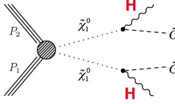
FIGURE 3. The \tilde{\chi}^0_1 \tilde{\chi}^0_1 decay to two Higgs bosons and \vec{E}_T^{\text{miss}}
