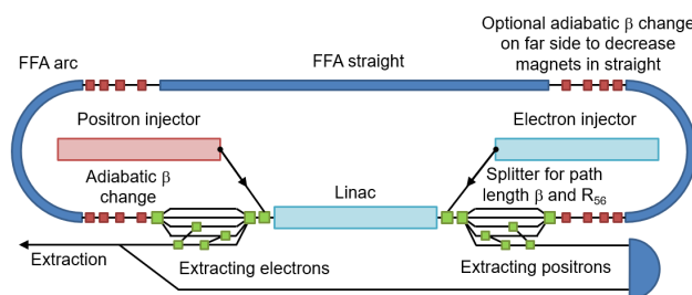
Figure 4: Proposed 1.2 GeV FFA booster for CEBAF.
