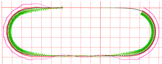
Figure 7: Orbits of 303, 404, 607, 809 and 1011 MeV particles in the FFA booster racetrack (10m grid shown). Orbits have been transversely exaggerated by 256x.
