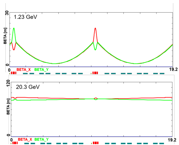
Figure 3: "Twin-Cell" periodic triplet lattice at the initial and final linac passes: 1.23 GeV and 20.3 GeV. Initial triplets, configured with 45 Tesla/m quads, are scaled with increasing momentum along the linac.
