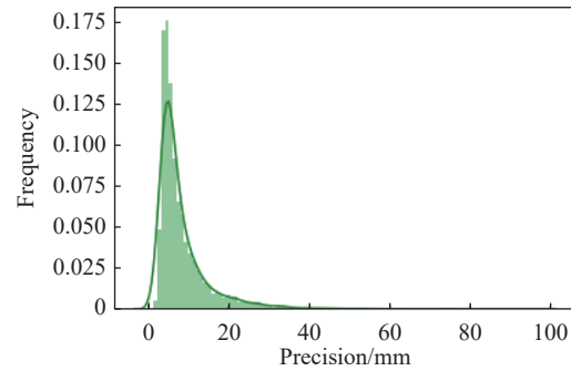
Fig. 12. The distribution of uncertainty in the APOLLO dataset.
