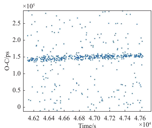
Fig. 19. Residuals of the measurement data of the Yunnan Observatory LLR.
