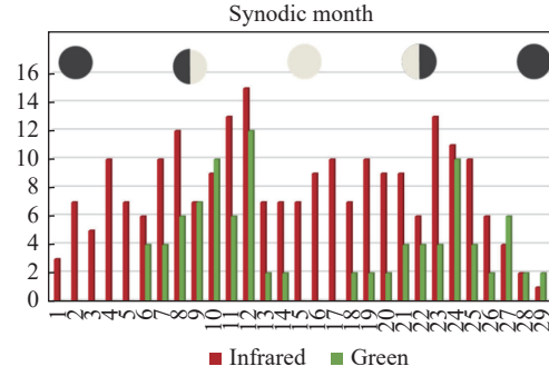
Fig. 17. Repartition of normal points during the synodic month [16] .
