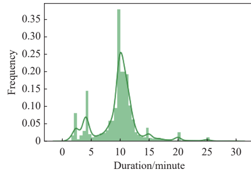
Fig. 8. Probability density distribution of Lunar Laser Ranging session duration.
