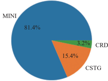
Fig. 9. The distribution of LLR Data Format in the LLR dataset.
