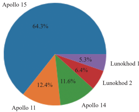
Fig. 5. The distribution of retro-reflectors in the LLR dataset.
