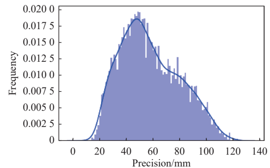
Fig. 14. The distribution of precision of returned photons in the Grasse dataset.
