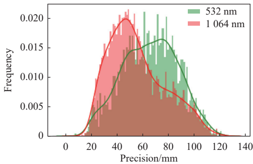
Fig. 15. The distribution of uncertainty in the Grasse dataset for lunar laser ranging using different laser wavelengths.
