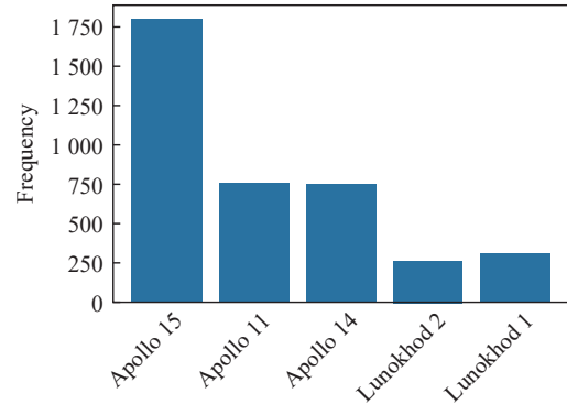
Fig. 11. The distribution of lunar retro-reflectors in the APOLLO dataset.
