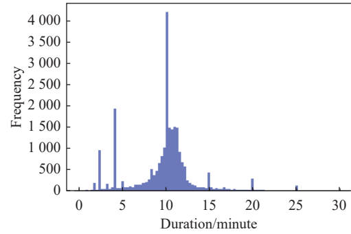
Fig. 7. Distribution of Lunar Laser Ranging session duration.
