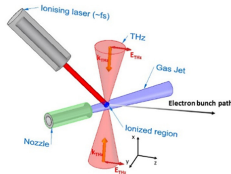
Figure 1: The schematic view of the proposed accelerator setup.
