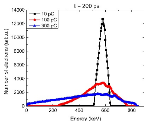
Figure 4: The energy spectra of the electron bunches after they ripped off from the ionized region (short cylinder).
