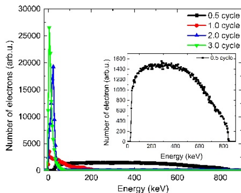
Figure 2: Energy spectra of the electrons (inset: Energy spectra of the electrons using “half” cycle THz pulses).
