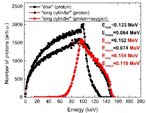
Figure 3: Comparison of the energy spectra of protons based on the two optimized setups.
