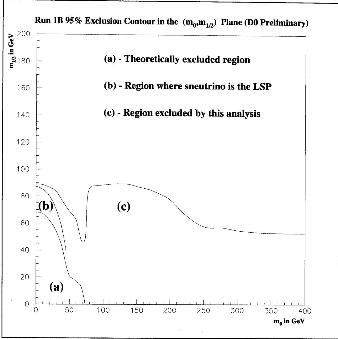
FIG. 1. 95% exclusion contour in the m_0 - m_{1/2} plane from the present analysis with \tan(\beta)=2 , A_0=0 and \text{sign}(\mu)=-1
