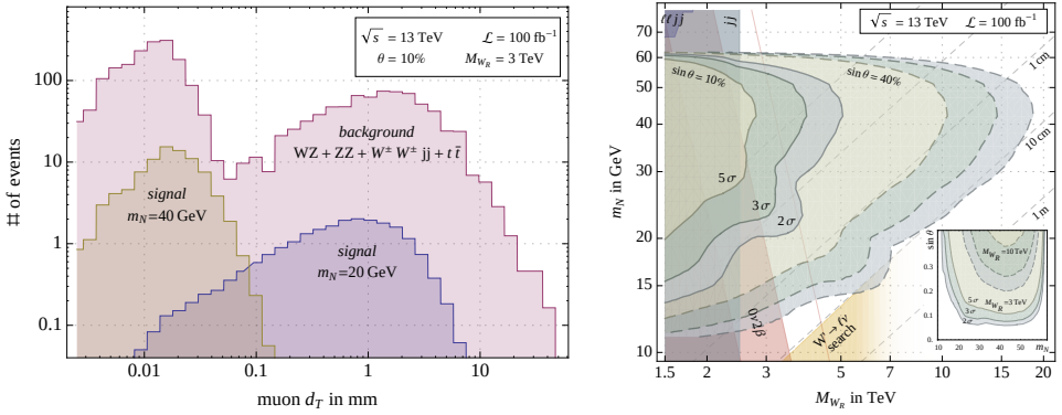
Fig. 1. Left: Transverse displacement of the muon vertex. Right: Contours of signal significance in \sigma_s for \theta = 10\% ( 40\% ) in solid (dashed) lines. Searches for the KS and di-jet channels (blue) and W_R \rightarrow \ell + \cancel{E} (yellow) are shown. Color on-line.
