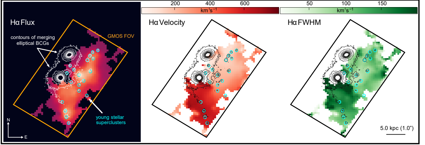
Figure 13. Left to Right: GMOS maps of H \alpha flux, line-of-sight velocity, and velocity dispersion, extracted after subtracting the stellar continuum as described in Section 2.3. White (left) and grey (center, right) contours depict the HST F606w view of the BCGs. Blue circles indicate the spatial location of the 19 young stellar superclusters (YSCs). The H \alpha -emitting gas fully engulfs the YSCs and may extend beyond the eastern edge of the GMOS FOV. The velocities shown are projected around a zero point at z = 0.335 (e.g., cz = 100,430 \text{ km s}^{-1} ), consistent with the velocity calibration used for the ALMA maps in Section 3.4.2. The gas is redshifted up to +800 \text{ km s}^{-1} with respect to the southern BCG and is most disturbed near the southern nucleus. We directly compare these kinematic maps with the ALMA data in Section 3.4.5.
