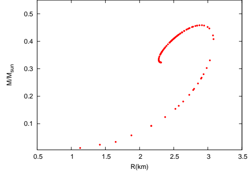
FIG. 1: The mass-radius relation of quark star
