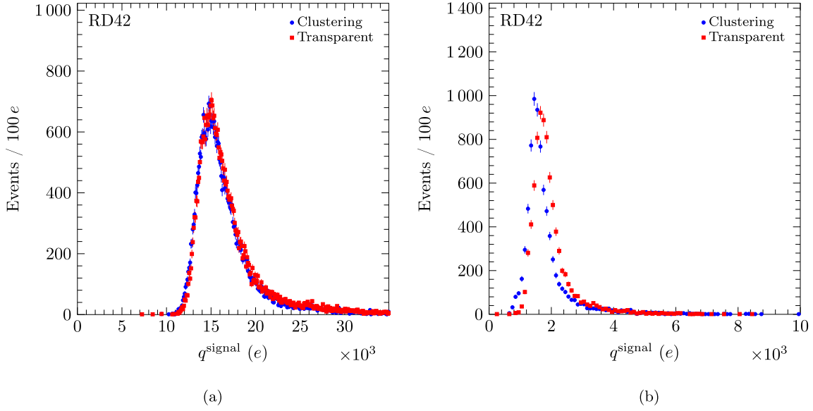
Figure 7. The signal charge distributions reconstructed with transparent and clustered algorithms (a) non-irradiated and (b) after an 800 MeV proton fluence of 13.4 \times 10^{15} \text{ p cm}^{-2} for sample 4.
