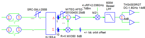
Figure 3: Modified bunch position detection circuit using cable-combined bandpass filters.
