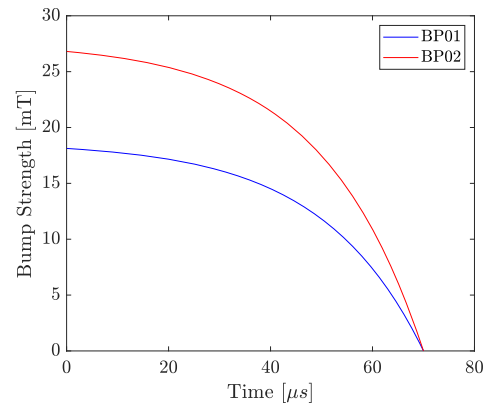
Figure 1: Injection bump magnet curves.
