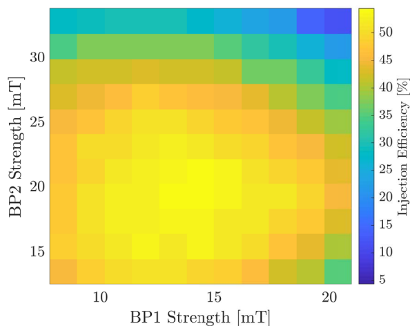
Figure 3: Injection bump strength scan.
