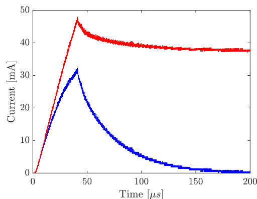
Figure 5: Injection current curve after adjustment of injector.
