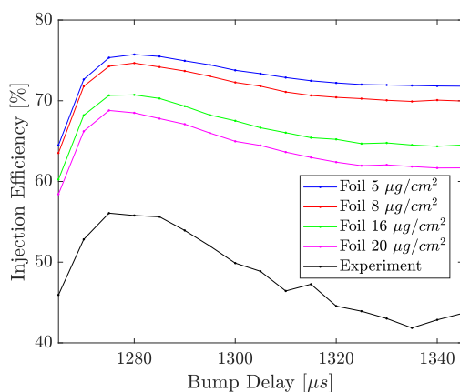
Figure 4: Injection bump delay scan.
