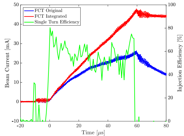
Figure 2: Injection current curve and single turn injection efficiency curve.
