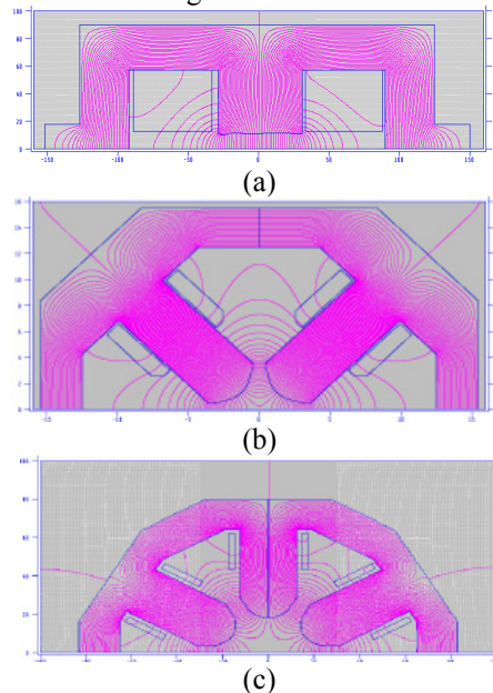
Figure 3: Design overview of the booster magnets.
