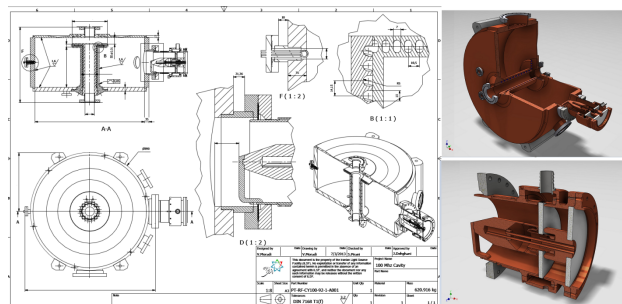
Figure 6: Mechanical drawing of designed cavity.
