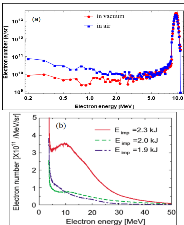
Figure 2: The electron energy spectrums of accelerator, (a) LINAC and (b) LWFA [3].
