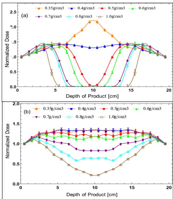
Figure 5: The depth-dose curve inside products irradiated double sided by electron beam (a) LINAC and (b) LWFA.
