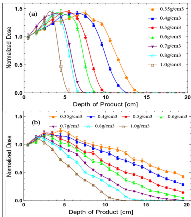
Figure 4: The depth-dose curve inside products irradiated one side by electron beam (a) LINAC and (b) LWFA.
