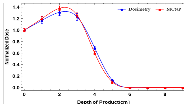
Figure 3: Depth-dose distribution inside the PP dummy irradiated by UELR-10-15S2 accelerator.
