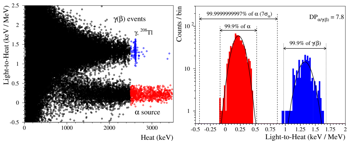
Figure 3. Left panel: Heat energy distribution of the light-to-heat parameter, L/H , of nuclear events detected by a scintillating bolometer based on a 379 g ^{100}\text{Mo} -enriched zinc molybdate crystal (enrZMO-t in [74]) and a thin Ge bolometric light detectors (LDs). First the detector was operated deep underground over 78 h of \gamma calibration and 593 h of background measurements. The crystal has been also irradiated by a ^{238}\text{U}/^{234}\text{U} \alpha source, emitting \alpha particles degraded in energy. The 2.5–3.5 MeV events, marked in blue and red, are used to illustrate the discrimination power parameter (see text). Right panel: Distributions of the L/H parameter of events selected from the data (shown in the left panel) in the 2.5–3.5 MeV energy interval [74]. Both distributions are fitted by Gaussian functions shown by solid lines. The intervals containing 99.9% of both event types and \pm 7\sigma range of the \alpha band are indicated. The discrimination power is evaluated as DP_{\alpha/\gamma(\beta)} = 7.8 (see text for details). Right panel is reprinted with permission from [74]. Creative Commons License CC BY 4.0.
