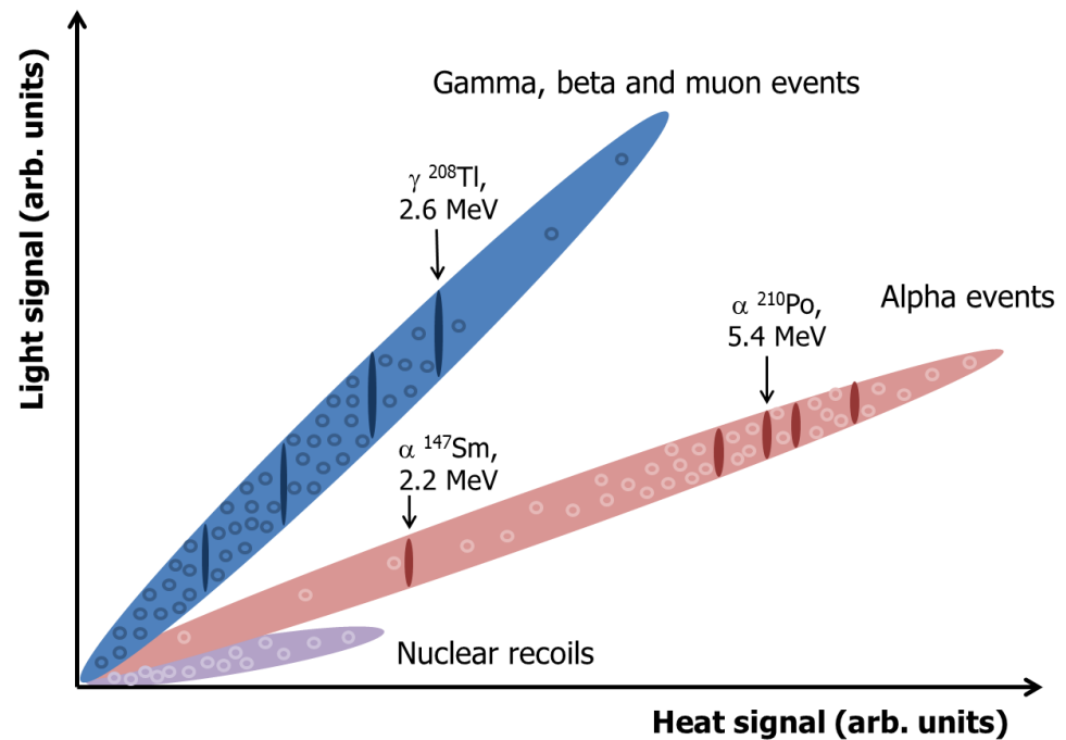
Figure 1. Schematic presentation of particle-dependent distributions of light signals measured by a photodetector in coincidences with the energy releases detected by a crystal scintillator-based bolometer. Circles represent individual events, which can form peaks shown as dark ovals on the \beta(\gamma, \mu) and \alpha bands. The light output induced by highly ionizing particles (alpha particles, nuclear recoils) impinging the scintillator is suppressed (quenched) with respect to the one induced by electrons (as well as \gamma quanta, cosmic-ray muons) of the same energy. Therefore, particles with different ionization properties become separated on such light vs. heat scatter-plot. The separation is more profound at higher energies, with increased amount of the detected scintillation light.
