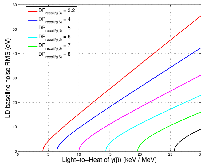
Figure 6. Discrimination power DP_{\text{recoil}/\gamma(\beta)} expected at 10 keV (an example of a possible dark matter search ROI), as a function of the LD noise resolution and the relative scintillation signal ( L/H_{\gamma(\beta)} ) parameter) of a scintillating bolometer. The assumed quenching factor for nuclear recoils (0.1) and an average photon energy (2.95 eV) are taken as for calcium tungstate scintillating bolometers.
