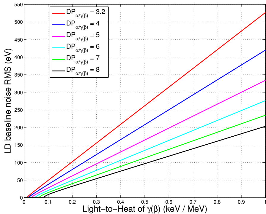
Figure 4. Discrimination power DP_{\alpha/\gamma(\beta)} expected at 3 MeV ( ^{100}\text{Mo} 0\nu\text{DBD} region-of-interest (ROI)) as a function of the LD noise resolution and the relative scintillation signal of a scintillating bolometer expressed by the L/H_{\gamma(\beta)} parameter. The used quenching factor for alpha particles (0.2) and an average photon energy (2.07 eV) are taken as for lithium molybdate scintillating bolometers.
