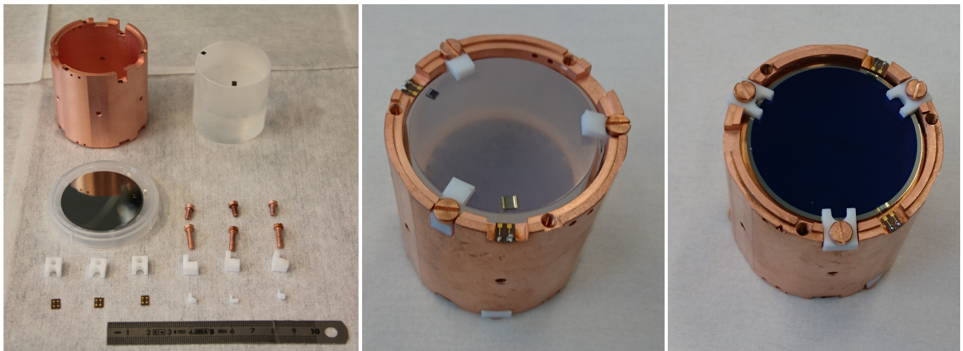
Figure 2. Left panel: A kit of components of a single detector module developed for the CUPID-Mo experiment with 20 scintillating bolometers to search for double-beta decay (DBD) processes in ^{100}\text{Mo} [159,259]. Each module is made of a Cu housing, a ^{100}\text{Mo} -enriched lithium molybdate crystal scintillator ( \varnothing 44 \times 45 mm, \sim 210 g) and a Ge wafer ( \varnothing 44 \times 0.2 mm, \sim 1.4 g) with glued small sensors, the Cu screws, the PTFE (polytetrafluoroethylene) spacers and fixing elements, and the Kapton ® film with Au pads. Middle panel: The assembled CUPID-Mo module, view from the top on the semi-transparent crystal surface with a Neutron-Transmutation-Doped Ge thermistor ( 3.0 \times 3.0 \times 1.0 mm) and a P-doped Si heater. A reflective film (Vikiuti TM ) has been put around the lateral side of the crystal. Right panel: The CUPID-Mo module, view from the bottom on the Ge disk equipped with the smaller thermistor ( 3.0 \times 0.8 \times 1.0 mm). The wafer is coated with a \sim 70 nm SiO layer (dark blue internal circle); the 2 mm on the edge of the wafer (17% of the area) remain uncoated. All photos are reprinted with permission from [259]. Creative Commons License CC BY 4.0.
