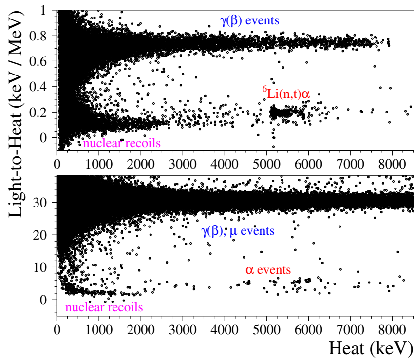
Figure 5. Energy distribution of the L/H parameter of nuclear events detected by scintillating bolometers based on a 213 g ^{100}\text{Mo} -enriched lithium molybdate (top panel; enrLMO-3 in [345]) and a 35 g ^{116}\text{Cd} -enriched cadmium tungstate (bottom panel; [346]), and both accompanied by a Ge LD. The data were acquired over 290 h of AmBe neutron calibration in an underground set-up (top panel) [345] and over 250 h of measurements (190 h of background and 60 h of \gamma calibration with a ^{232}\text{Th} source) in an aboveground laboratory (bottom panel) [346]. Bottom panel is reprinted with permission from [346]. Creative Commons License CC BY 4.0.
