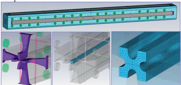
Figure 4: The MWS RFQ model.
