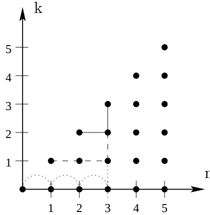
Fig. 1. Illustration of the connections between the coefficients of the scalar two-point function in the spontaneously broken phase of the linear sigma model at order g_r^3 . The quantity n represents the order in g_r and k stands for the exponent of the logarithm L_s . Every type of line indicates recursion relations which contain the connected coefficients. The solid line corresponds to Eq. (1). There is one such picture for every order in \frac{s}{m_r^2} .
