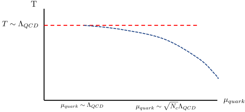
Fig. 2. (Color online) The deconfinement temperature in this plot is the long-dashed red line for infinite N_c and the dashed blue line for finite but large N_c .
