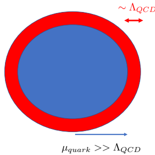
Fig. 4. (Color online) A Fermi sphere of quarks (inner/blue) surrounded by a shell of nucleonic matter (outer/red).
