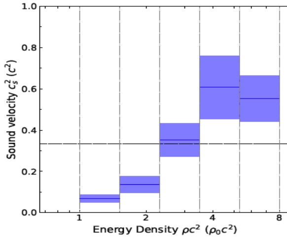
Fig. 6. The sound velocity as a function of density from the analysis of Fujimoto et al. [9].
