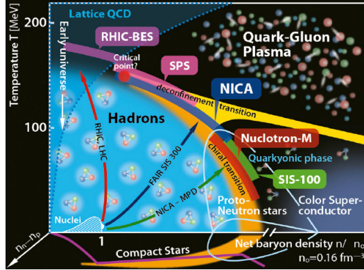
Fig. 1. A popular hypothetical diagram showing possible phases of QCD [1].
