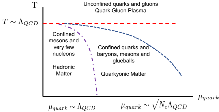
Fig. 3. A phase diagram of QCD appropriate for large N_c that includes Quarkyonic Matter.
