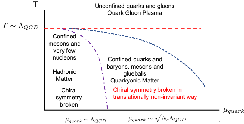
Fig. 5. A hypothetical phase diagram of QCD in the large- N_c limit.
