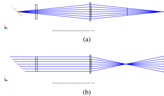
Figure 1: Single HRFZ Si lens imaging system in a 2f - 2f setup imaging a TR target at 45^\circ . Top: CTR ray diagram. Bottom: upstream source (e.g. CSR) ray diagram.
