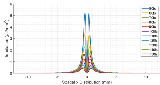
Figure 2: Example simulated CTR image profiles using the system shown in Fig. 1.
