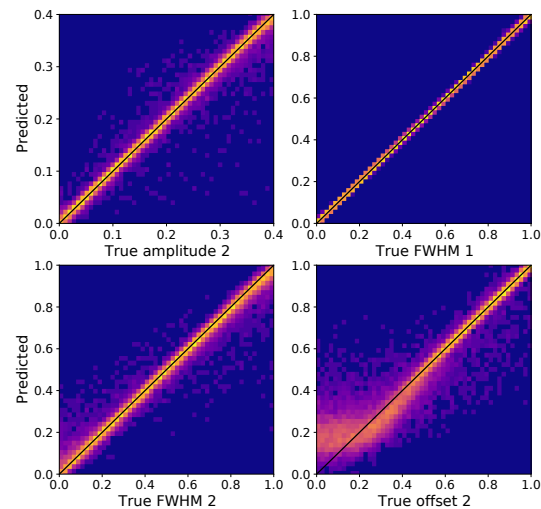
Figure 5: Initial validation results of the new neural network model for CTR image analysis.
