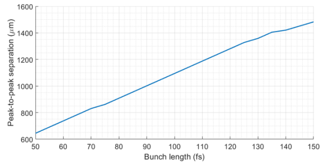
Figure 3: Typical analysis of the images presented in Fig. 2. CTR image width variation with bunch length.
