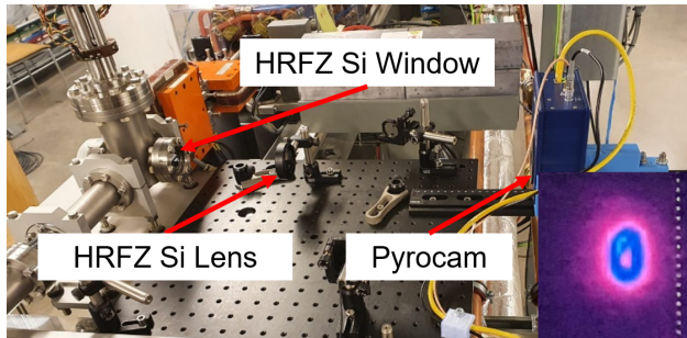
Figure 4: HRFZ Si system at the MAX IV SPF. Inset image is the first test image of CTR with the system.
