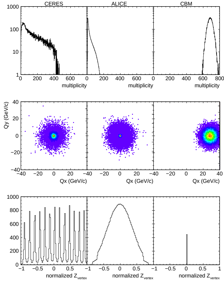
Fig. 2. Global observables: raw multiplicity (top), flow vector (middle), and the longitudinal position of the event vertex (bottom) for CERES, ALICE, and CBM (left, middle and right, respectively). Counts were scaled arbitrarily.
