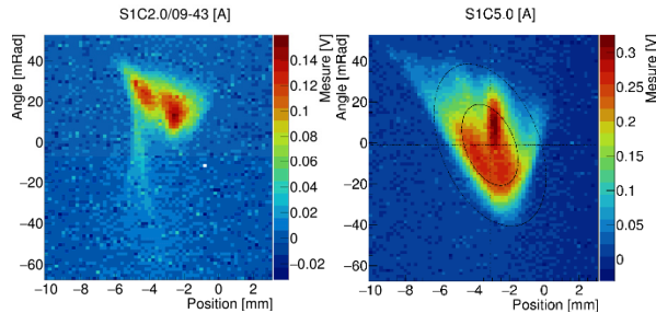
Figure 3: (x,x') Distribution of the H - beam. On the left, the source current (S1C) is fixed at 2 A. It is the start-up reference beam. On the right, one of the measurements for the arc current ramped up to S1C=5 A. Also, 1 and 2- \sigma ellipses are drawn, with the centroid (cross).
