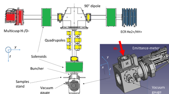
Figure 1: The emittance-meter in the injection beamline above the cyclotron.
