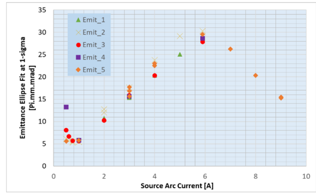
Figure 4: Emittances as given by a 1- \sigma fit ellipse for five scans of the source arc current performed on different days.
