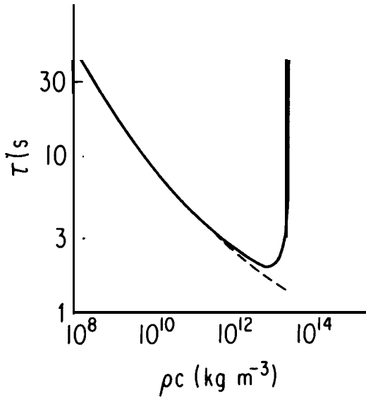
Fig. 6. The variation of the period of radial oscillation along the completely degenerate configurations. Notice that the period tends to infinity for a mass close to the limiting mass. There is consequently a minimum period of oscillation along these configurations; and the minimum period is approximately 2 seconds. (From J. Skilling, Pulsating Stars (Plenum Press, New York, 1968), p. 59.)
