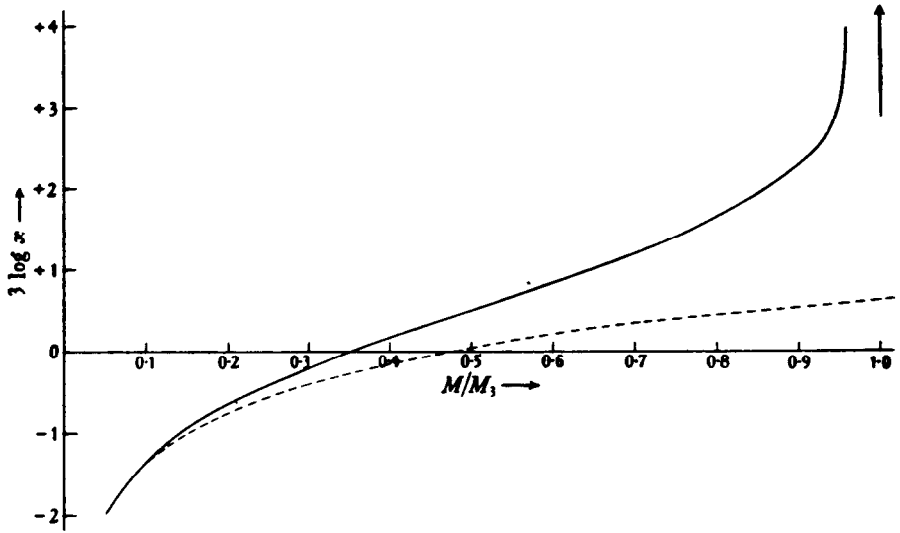
Fig. 3. The full-line curve represents the exact (mass-density)-relation for the highly collapsed configurations. This curve tends asymptotically to the dotted curve as M \rightarrow 0 . (From Chandrasekhar, S., Mon. Not. Roy. Astr. Soc. , 95, 207 (1935).)
