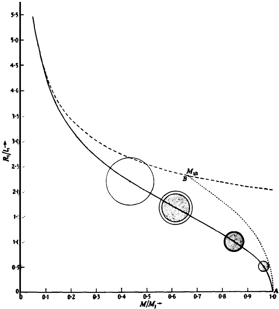
Fig. 2. The full-line curve represents the exact (mass-radius)-relation ( L_e is defined in equation (46) and M_1 denotes the limiting mass). This curve tends asymptotically to the ---- curve appropriate to the low-mass degenerate configurations, approximated by polytropes of index 3/2. The regions of the configurations which may be considered as relativistic ( \rho > (K_1/K_2)^3 ) are shown shaded. (From Chandrasekhar, S., Mon. Not. Roy. Astr. Soc. , 95, 207 (1935).)
