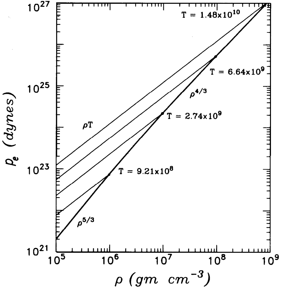
Fig. 4. Illustrating how by increasing the density at constant temperature degeneracy always sets in.
