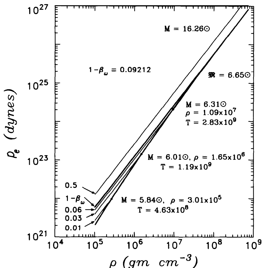
Fig. 5. Illustrating the onset of degeneracy for increasing density at constant \beta . Notice that there are no intersections for \beta > 0.09212 . In the figure, 1 - \beta is converted into mass of a star built on the standard model.
