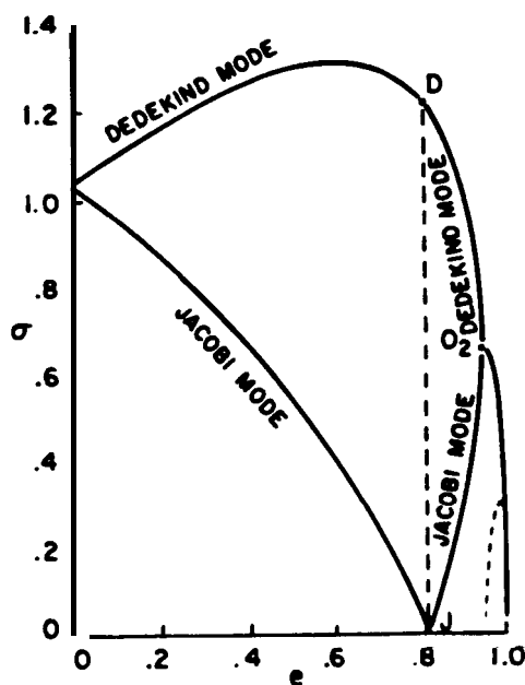
Fig. 7. The characteristic frequencies (in the unit (\pi G \rho)^{1/2} ) of the two even modes of second-harmonic oscillation of the Maclaurin spheroid. The Jacobi sequence bifurcates from the Maclaurin sequence by the mode that is neutral ( \sigma = 0 ) at e = 0.813 ; and the Dedekind sequence bifurcates by the alternative mode at D. At O_2 ( e = 0.9529 ) the Maclaurin spheroid becomes dynamically unstable. The real and the imaginary parts of the frequency, beyond O_2 are shown by the full line and the dashed curves, respectively. Viscous dissipation induces instability in the branch of the Jacobi mode; and radiation-reaction induces instability in the branch DO_2 of the Dedekind mode.
