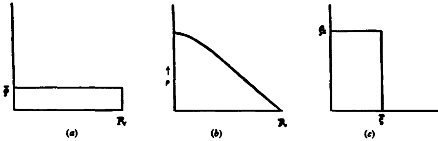
Fig. 1. A comparison of an inhomogeneous distribution of density in a star (b) with the two homogeneous configurations with the constant density equal to the mean density (a) and equal to the density at the centre (c).
