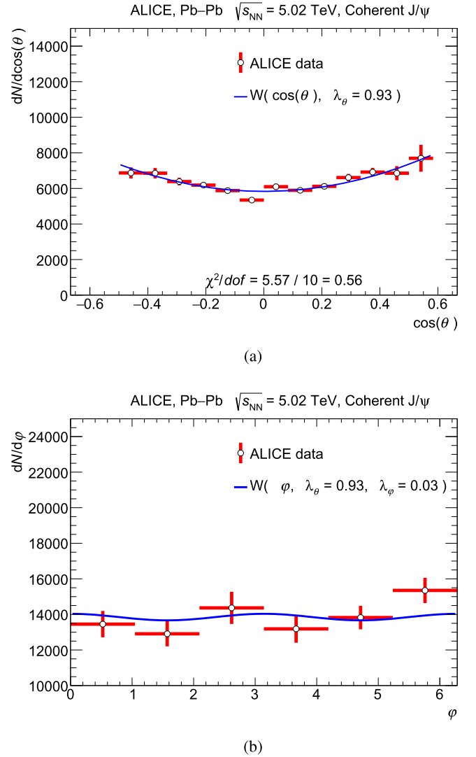
Fig. 3. Projections of the coherent J/\psi data points in (a) \cos\theta and (b) \varphi , for events in the -4 < y < -2.5 rapidity interval. The curves are obtained by setting the lambda parameters in Eq. (2) to the results of the fit to the distribution given in Table 2. The uncertainties on the data points are statistical.
