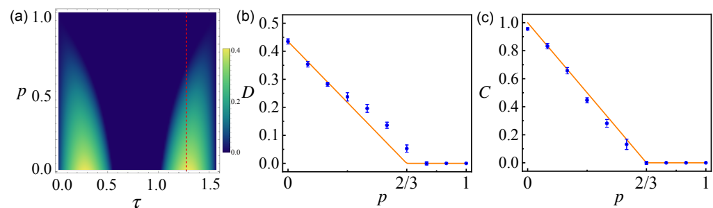
Figure 3. Performance of the protocol for mixed entangled states. (a) Numerical analysis of D dependence of p and \tau . The density is colored according to the degree of the distance D . The dashed red line indicates \tau = \frac{13}{32}\pi . (b) Results of performing the protocol for detecting initial entanglement. \tau is fixed to \frac{13}{32}\pi such that \rho_{SE} is always detected as entangled as long as p < \frac{2}{3} ; then, the protocol ends in good agreement with that of directly detecting \rho_{SE} via 2-qubit QST, as shown in (c). (c) Concurrence of the initial states \rho_{SE} for different state parameters p , obtained via 2-qubit QST.
