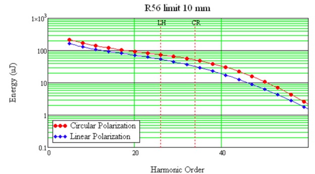
Figure 4: Output pulse energy for FEL-1 in EEHG operation mode (red-blue for circular (C) and linear (L) polarizations) . FEL-1 present configuration: six undulator modules, 2.2 m long, 5 cm of period length.
