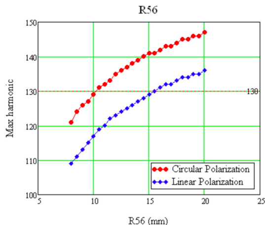
Figure 3: Maximum harmonic order reaching saturation vs. the first chicane dispersion in EEHG configuration.
