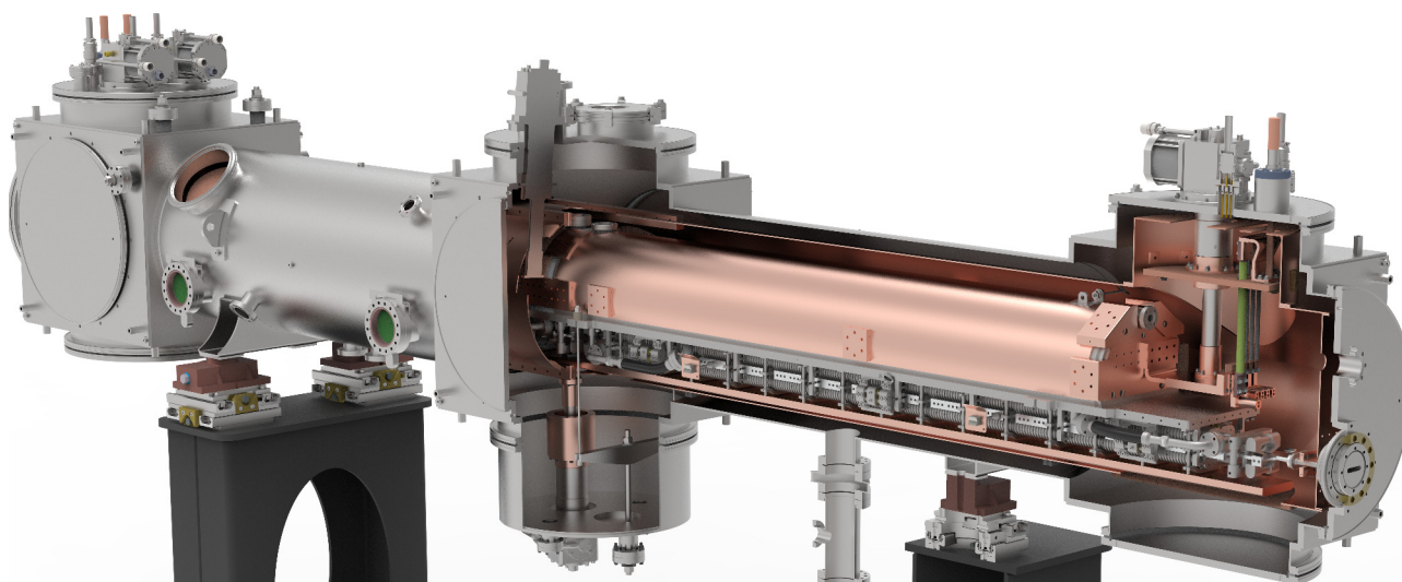
Figure 2: Rendering of the 4.8-meter long SCU cryostat with a portion of the vacuum vessel and thermal shield cut away to expose the cold mass.
