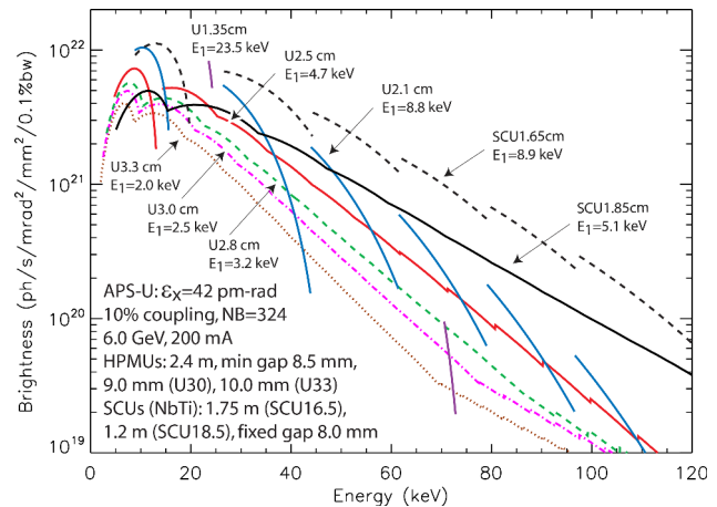
Figure 1: Calculated brightness tuning curves of odd harmonics of most hybrid permanent magnet undulators and SCUs for APS-U.
