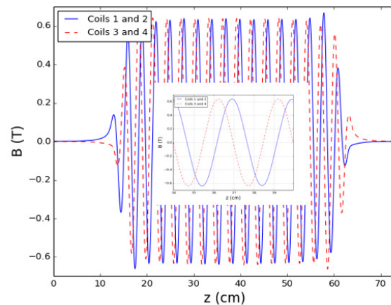
Figure 5: Magnetic measurement of the 0.5-meter long SCAPE prototype in circular mode. Inset is a two period close-up of the data showing the 1/4 period shift between the orthogonal magnets.
