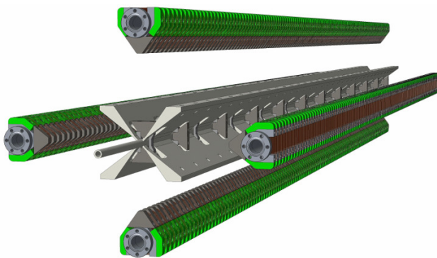
Figure 4: Exploded view of the SCAPE magnet with the beam vacuum chamber [10].
