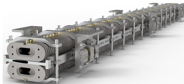
Figure 3: Model of the planar SCU magnetic assembly and beam vacuum chamber.
