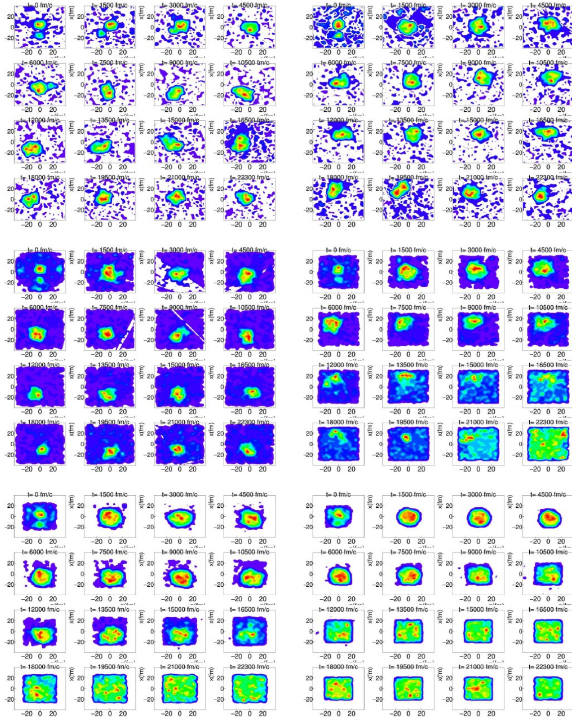
Figure 2. Evolution of the system ^{140}\text{Ni}+^{460}\text{U} in the nucleon bath with 10% proton concentration calculated using the CoMD code at beam energy 0.01\text{MeV/nucleon} and Coulomb interaction cutoff at 10, 7, 5, 4, 3, and 2 fm (from top to bottom and left to right), corresponding to nucleon bath densities \rho_0/100 , \rho_0/50 , \rho_0/30 , \rho_0/17 , \rho_0/10 , and \rho_0/5 , respectively. Incompressibility is K_0 = 254\text{MeV} and a soft density dependence of symmetry energy were used. The initial distance is 25 fm. On the time scale up to 25000 fm/c the resulting nucleus appears to dissolve in the nucleon bath with density above \rho_0/30 , even sooner with increasing density.
