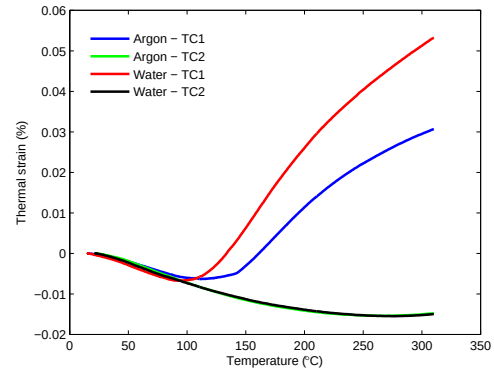
Figure 3: Thermal cycling following irradiation of 3D C/C composite specimens.
