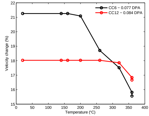
Figure 6: Ultrasonic velocity recovery in irradiated and annealed C-2020 specimens.
