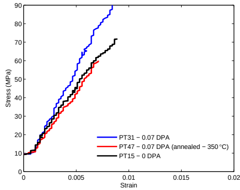
Figure 5: Annealing effect on tensile properties of POCO.
