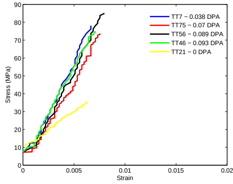
Figure 4: Stress strain curves for irradiated IG-430 at varying DPA levels.
