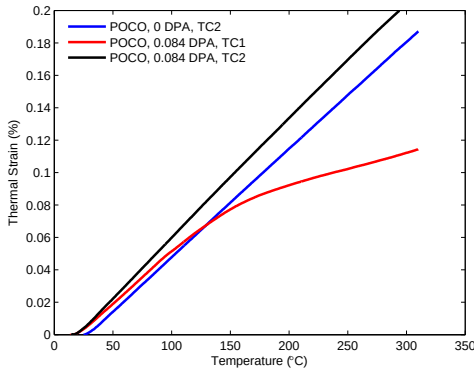
Figure 2: Dimensional changes in un-irradiated and irradiated POCO graphite over two thermal cycles.
