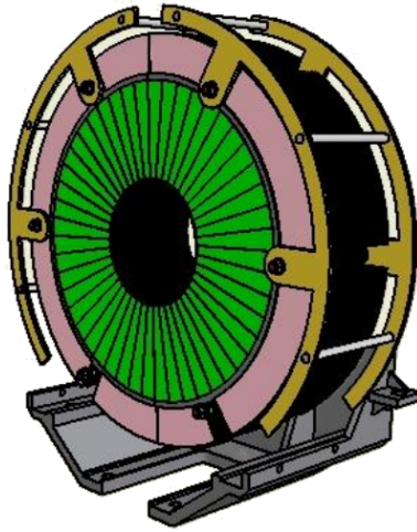
Fig. 2. A schematic drawing of LumiCal detector.
