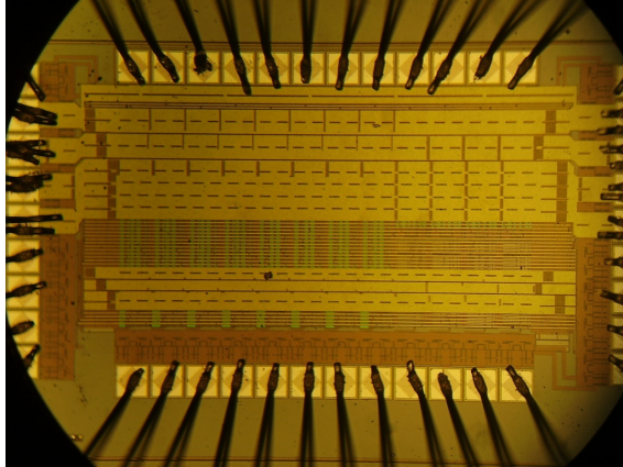
Fig. 5. A micrograph of a front-end ASIC.
