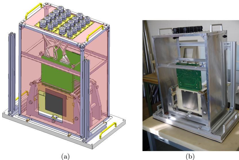
Fig. 8. (a) Schematic diagram of the precise mechanical frame. (b) Photograph of the frame prototype with absorber plate and detector module inserted.
