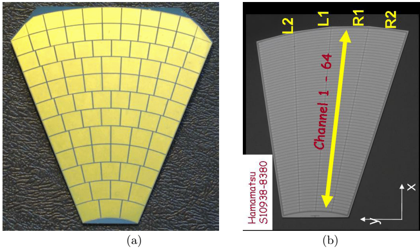
Fig. 4. (a) A prototype of a GaAs sensor sector for BeamCal. (b) The layout of a sensor tile for LumiCal. L1, L2, R1, R2 mark four sectors of a single tile.
