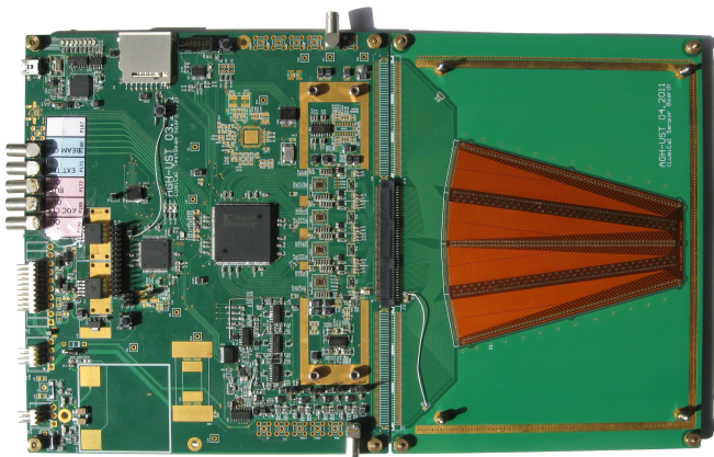
Fig. 3. Photograph of a LumiCal readout module with sensor connected.
