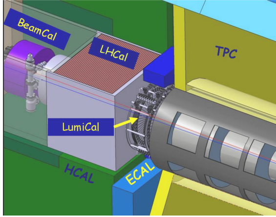
Fig. 1. The very forward region of the ILD detector, containing the BeamCal and LumiCal calorimeters.
