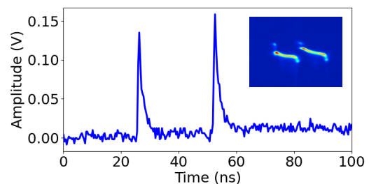
Figure 2: Fast diode waveform of the two laser heated pulses of about 30 ns apart. The inset contains the time-resolved longitudinal phase-space image.
