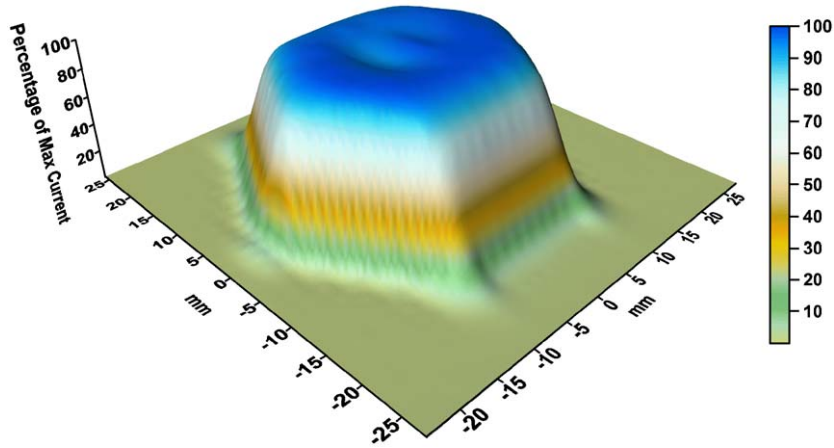
Fig. 7. Response uniformity for a hexagonal concave tile.
