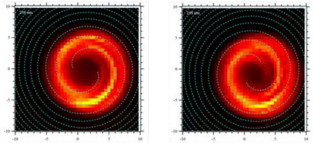
Figure 4: Interference pattern observed by scanning the fiberscope spectrometer. Upstream U: linear 1 st harmonic, Downstream U: circular 3 rd harmonic. E=500 MeV, \varepsilon_0=8 nm-rad, \lambda=248 nm. Dotted spiral line represents the calculated pattern with the extended equation based on that in ref. 11.
