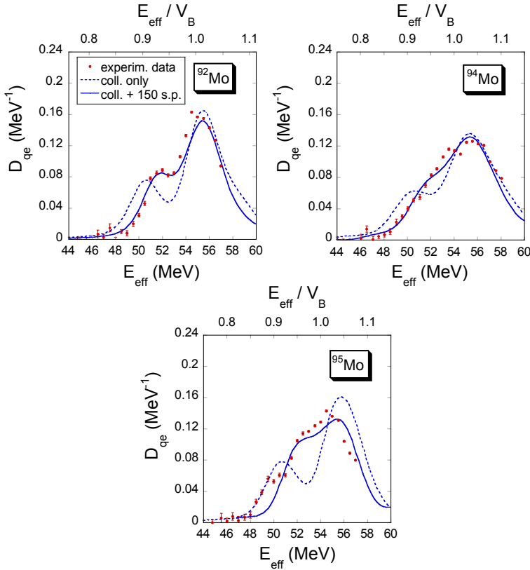
Fig. 2. Quasielastic barrier distributions of the ^{20}\text{Ne} + ^{92,94,95}\text{Mo} systems. The experimental data are compared with predicted barrier distributions, with (solid lines) and without including dissipation due to non-collective excitations (dashed lines). The energy resolution for the three systems was taken into account by folding the calculated distributions with a Gaussian function with a correspondent FWHM.
