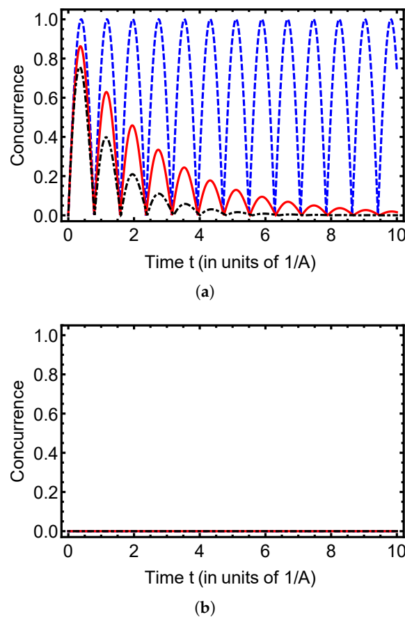
Figure 1. Evolution of the concurrence C(t) as a function of the time t (in units of 1/A ) for the initial separable state ( \alpha = 0 ) under different dephasing rates \Gamma . The curves correspond to \Gamma = 0 (dashed), \Gamma = 0.4A (solid), and \Gamma = 0.8A (dash-dotted). Panel (a) shows the dynamics for the initial state |\Psi(0)\rangle = |\uparrow_e\downarrow_p\rangle , while panel (b) corresponds to |\phi(0)\rangle = |\uparrow_e\uparrow_p\rangle . Here A denotes the hyperfine coupling constant, and \Gamma = \gamma_e + \gamma_p is the total dephasing rate due to electron and proton contributions.
