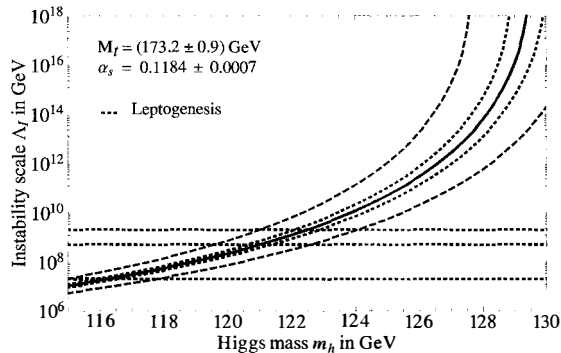
Figure 2: In red, the SM instability scale \Lambda_I as a function of the Higgs mass. The central curve correspond to M_I = 173.2 GeV and \alpha_s(M_Z) = 0.1184 and the side-bands to 1-sigma deviations (with larger deviation for the top mass). In black, the three dashed lines correspond to the lower limits of the mass of the lightest right-handed neutrino coming from thermal leptogenesis. The green band is the experimentally favoured Higgs mass.
