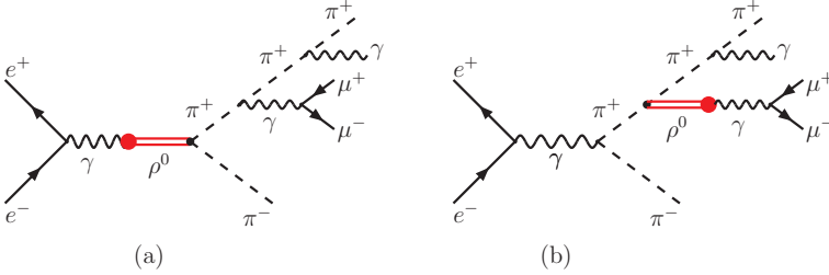
Fig. 2. Feynman diagrams of e^+e^- \rightarrow \pi^+\pi^-\mu^+\mu^-\gamma with \gamma - \rho^0 mixing.
