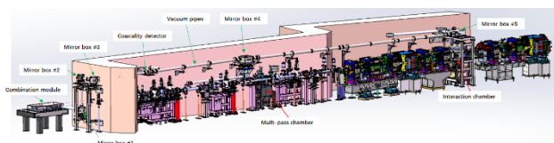
Figure 1: Laser transport system's layout over the frontend facilities and magnet lattice.
