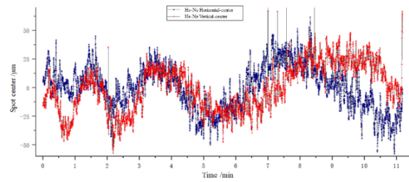
Figure 7: The jitter of the fitting results of He-Ne spot's center before entering multi-pass chamber.
