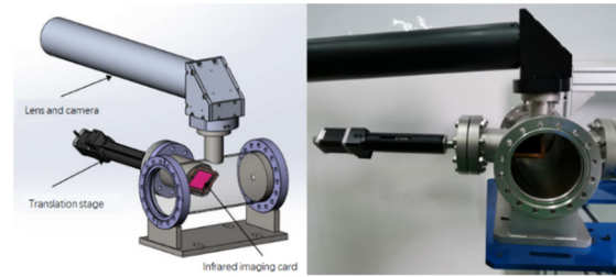
Figure 4: Coaxial detector's model (left) and photo (right).
