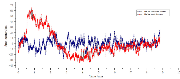
Figure 8: The jitter of the fitting results of He-Ne spot's center before entering interaction chamber.
