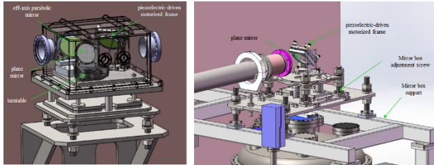
Figure 3: Piezoelectric-driven motorized frame in mirror box #4 (left) and #5 (right).
