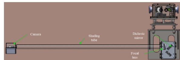
Figure 5: Direction detectors of laser's layout under mirror box #4.
