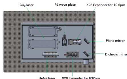
Figure 2: Laser combination module's layout.
