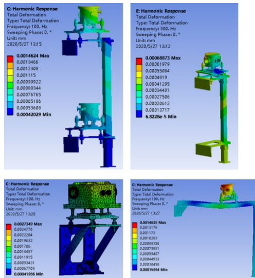
Figure 6: Harmonic response simulation results of the mirror box #1, #2 (upleft), #3 (upright), #4 (downleft), #5 (downright) with their support.
