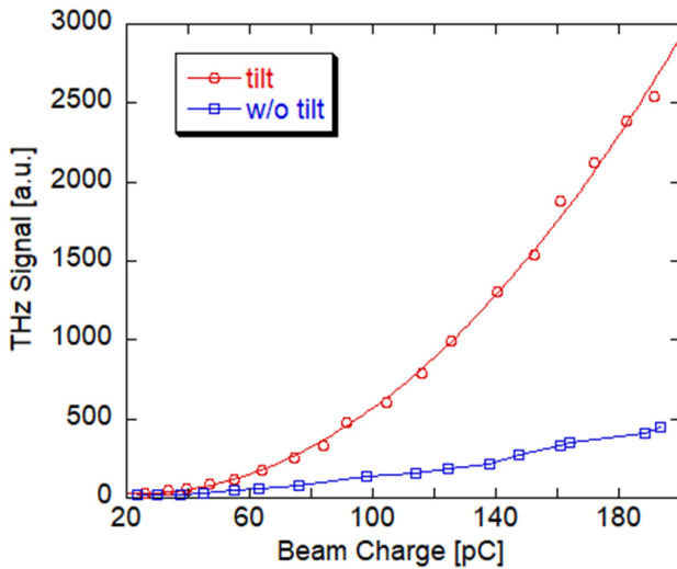
Figure 2: THz signal. The red line is the THz intensity of electron beam with tilt. The blue line is the THz signal of electron beam without tilt. THz signal of titled electron beam is proportional to the square of the number of electrons obviously.
