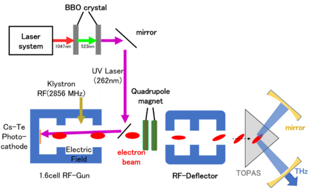
Figure 4: Experimental setup.
