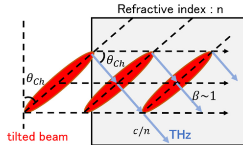
Figure 1: Phase matching coherent Cherenkov radiation.
