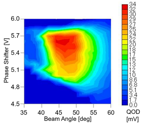
Figure 3: Radiation intensity measured by QOD with 0.5 THz band pass filter.
