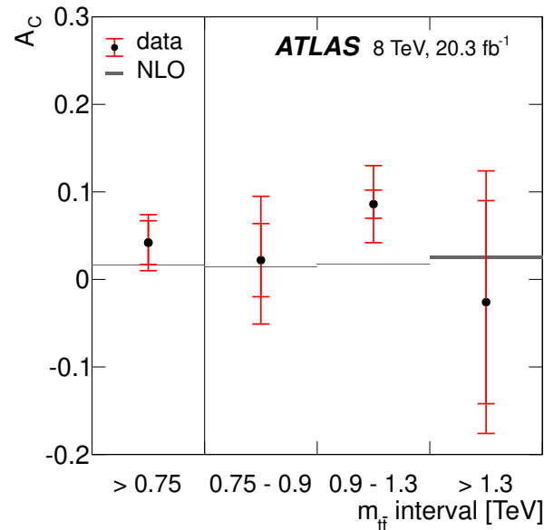
Figure 15. A_C^{t\bar{t}} values from the unfolded distributions as a function of m_{t\bar{t}} [48] compared to NLO calculation [13].
