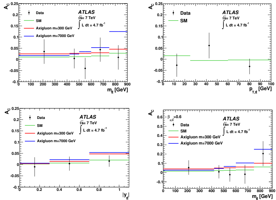
Figure 6. Distributions of A_C^{t\bar{t}} as a function of m_{t\bar{t}} (top left), p_{T,t\bar{t}} (top right), and |y_{t\bar{t}}| (bottom left) after unfolding, for the electron and muon channels combined. The A_C^{t\bar{t}} distribution as a function of m_{t\bar{t}} for \beta_{z,t\bar{t}} > 0.6 , is also shown (bottom right). The A_C^{t\bar{t}} values after the unfolding (points) are compared with the SM predictions (green lines) and the predictions for a colour–octet axigluon with a mass of 300 GeV (red lines) and 7000 GeV (blue lines), respectively. The thickness of the lines represents the factorization and renormalization scale uncertainties in the corresponding theoretical predictions. The values plotted are the average A_C^{t\bar{t}} in each bin. The error bars include both the statistical and the systematic uncertainties [29].
