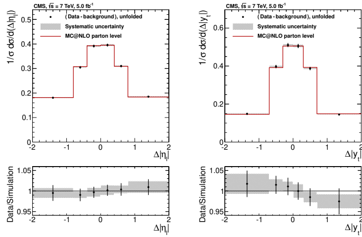
Figure 4. Background-subtracted and unfolded differential measurements of \Delta|\eta| ( left ) and \Delta|y| ( right ), both normalised to unit area (points), and the parton-level predictions from MC@NLO (histograms). Bottom: the ratio between the data and the MC@NLO prediction for lepton \Delta|\eta| ( left ) and \bar{t}\bar{t} \Delta|y| ( right ). The error bars represent the statistical uncertainties in the data, while the systematic uncertainties are represented by the hatched band. The first and last bins include underflow and overflow events, respectively [24].
