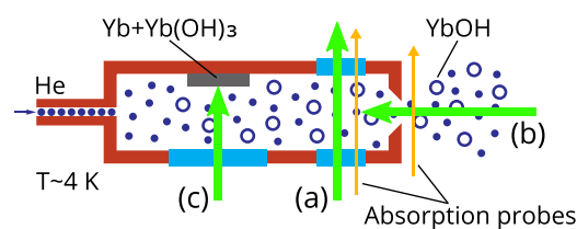
Figure 1. Depictions of the enhancement light geometries investigated. The enhancement light is depicted by the thick green arrows. The thin arrows indicate the absorption probes, which are fixed in position. (a) Transverse geometry: the enhancement light is introduced through a window \sim 25 mm away from the ablation target and \sim 12 mm away from the cell aperture. (b) Longitudinal geometry: the enhancement light is introduced through the cell aperture. (c) Collinear geometry: the enhancement light is sent through the ablation window, collinear with the YAG pulse.
