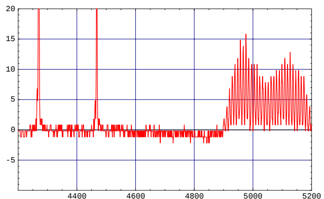
Figure 2. A histogram of the counts in the E0LTOT counter. The time bins are 2 ns and only a fraction of a turn is shown. To the left are two proton bunches and on the right are the counts caused by the TEL extracting protons that have drifted into the abort gap.
