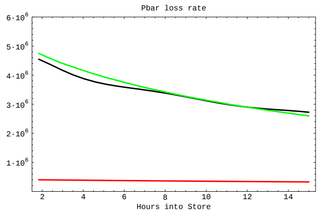
Figure 4. The top black curve is the total pbar loss rate. The top green/grey curve represents the loss due to pbar-p interactions, and the bottom curve is loss in the residual gas.
