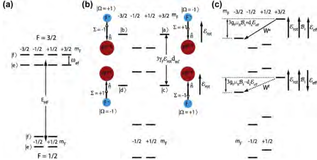
Figure 1.4 – Energy level structure of \text{HfF}^+ in the ^3\Delta_1(J=1) state including the hyperfine shifting respectively in the absence of electric field (a), in the presence of an external electric field (b) and under the application of a magnetic field in addition to the electric field and the existence of a permanent eEDM (c) [LBL + 11].
