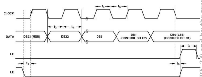
Figure 6: Timing diagram.
