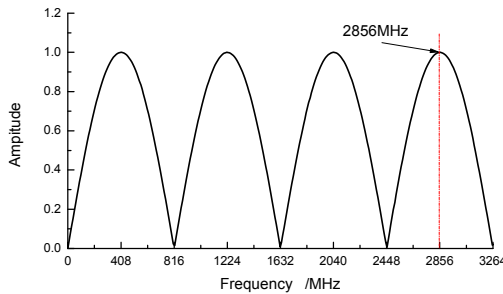
Figure 3: The frequency response of the stripline BPM.
