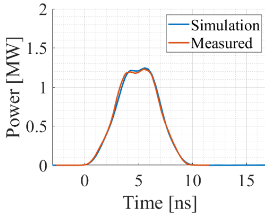
Figure 2: Measured (red) and simulated (blue) transmitted power through the DDA during low power operation.
