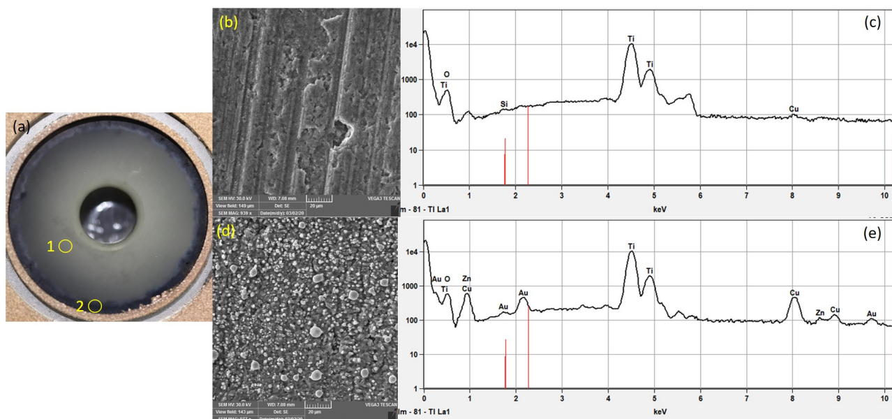
Figure 5: Photo of the interior face of one BaTi disk (a). SEM and EDX data were collected at locations indicated by the numbered circles: 1 corresponds to (b & c), and 2 to (d & e).
