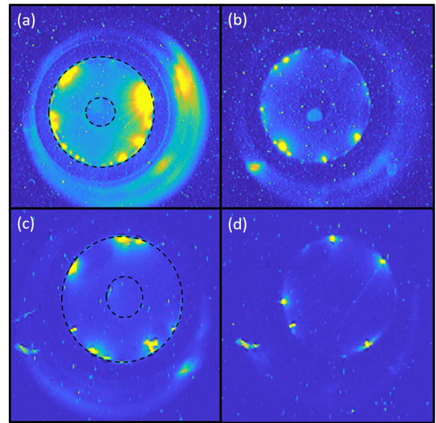
Figure 3: Snapshots of the face of the upstream (a & b) and downstream (c & d) disks, taken at the beginning (a & c) and end (b & d) of conditioning. The extents of the ceramic marked with dashed black lines on the left.
