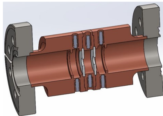
Figure 1: Cutaway view of the mechanical design of the DDA showing the dielectric cell and two matching metallic cells.
