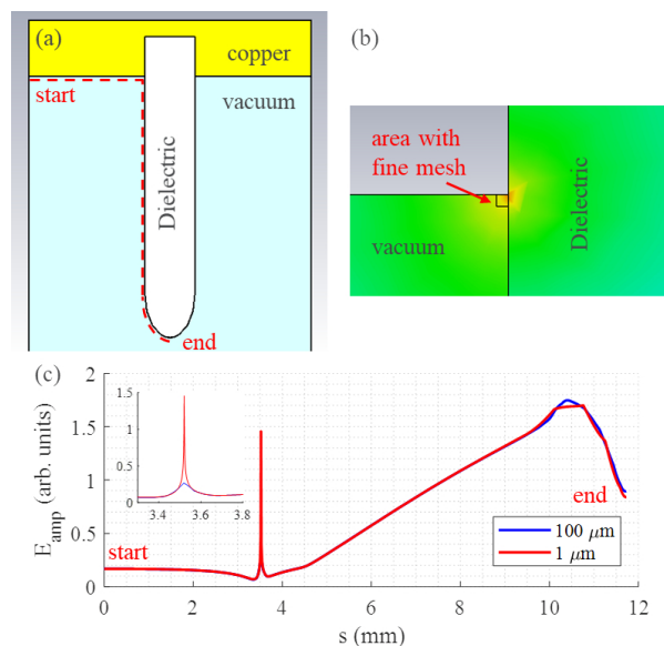
Figure 6: Increased mesh density at the triple junction (b) revealed field enhancement at the braze joint (a & c) comparable to that on the ceramic iris.
